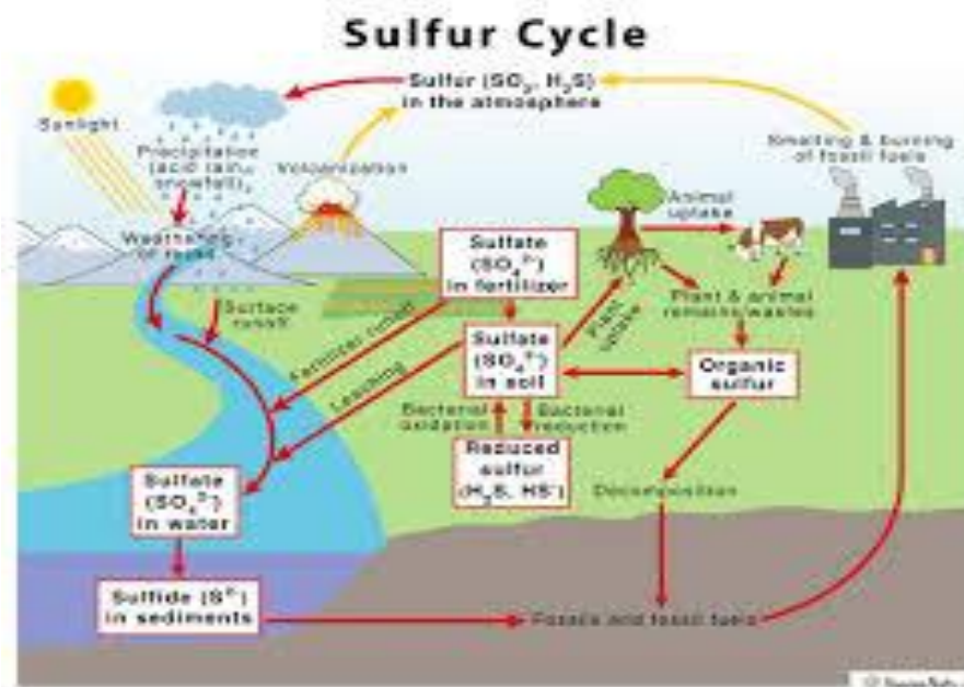
Figure 1c: Sulphur Cycle
