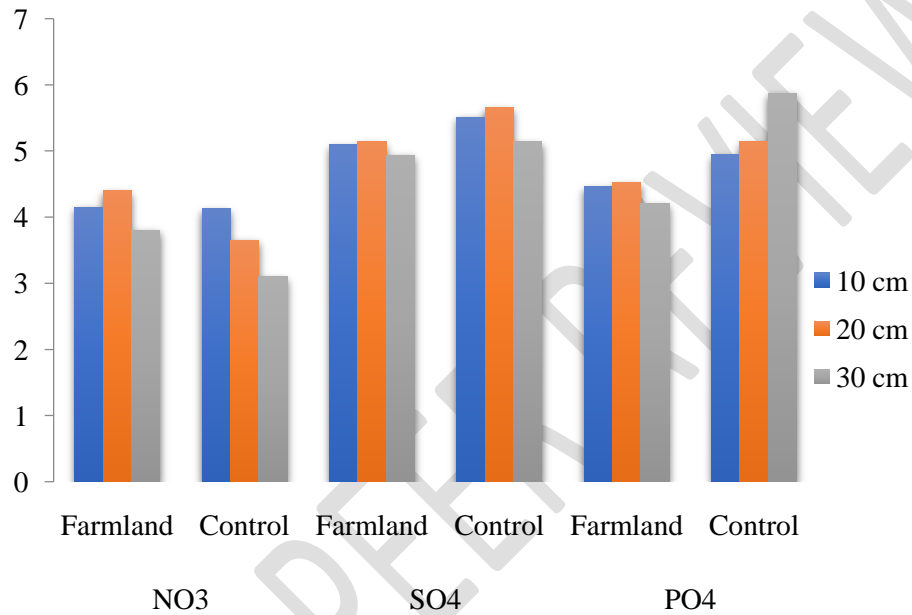
Figure 4: Chart showing the \text{NO}_3^- , \text{SO}_4^{2-} and \text{PO}_4^{3-} levels of soil samples collected from different depth in Kaiama farmland and control for November, 2021.
