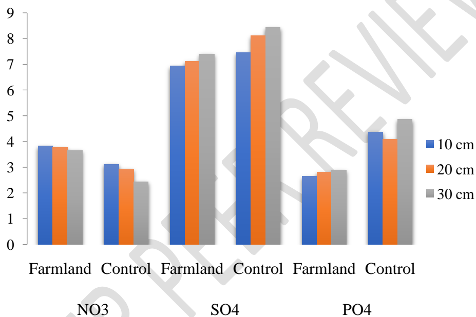
Figure 3d: Chart showing the \text{NO}_3^- , \text{SO}_4^{2-} and \text{PO}_4^{3-} levels of soil samples collected from different depth in Imiringi farmland and control for October, 2021
