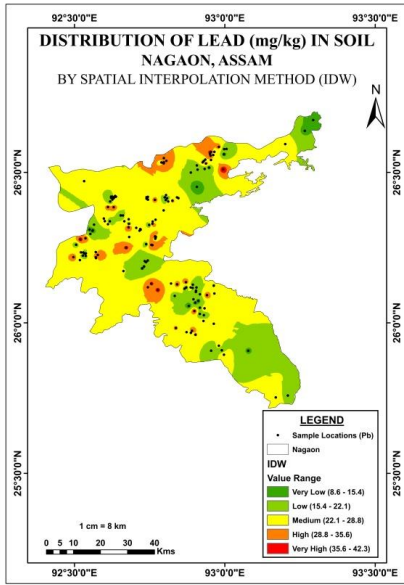
Fig 9: Soil Lead content (mg/Kg) across the district
