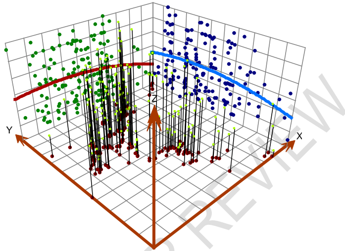
Fig 13: Trend analysis for Lead distribution in soil across the district
