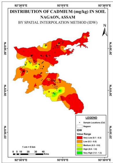
Fig 2: Soil Cadmium content (mg/Kg) across the district
