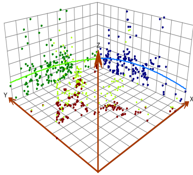
Fig 6: Trend analysis for Cadmium in soil
