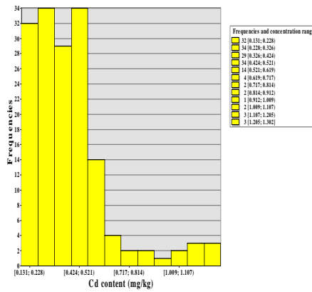
Fig 3 : Frequency and concentration range of Cadmium in
