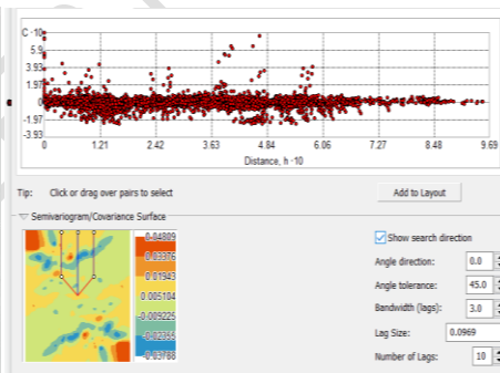
Fig 8: Covariance cloud of Cadmium in soil
