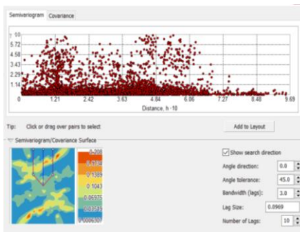
Fig 7: Semivariogram cloud of Cadmium in soil
