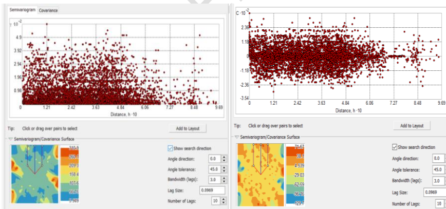
Fig 14: Semi-variogram for Lead distribution in soil
