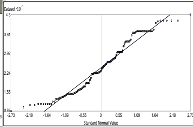
Fig 12: Normal Q-Q plot for Lead in soil
