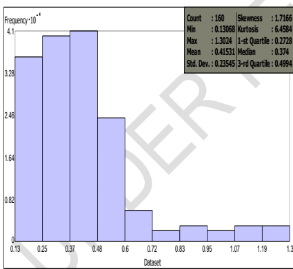
Fig 4: Histogram for lead content in soil
