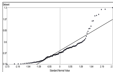
Fig 5: Normal Q-Q plot for Cadmium in soil
