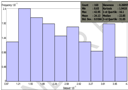
Fig 11: Histogram for lead content in soil
