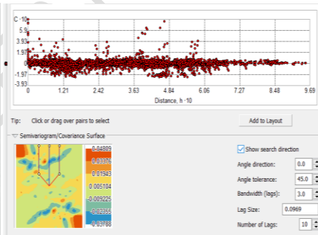
Fig 8: Covariance cloud of Cadmium in soil
