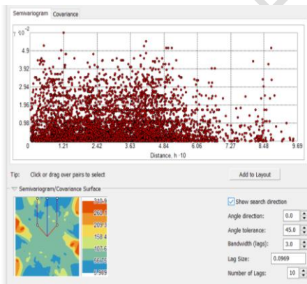
Fig 14: Semi-variogram for Lead distribution in soil
