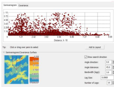
Fig 7: Semivariogram cloud of Cadmium in soil
