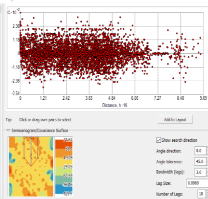
Fig 15: Co-variance cloud for Lead distribution in soil
