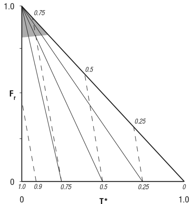
Figure 3. Right triangle with isopleths of M_o (thin sloping lines leaning left and labeled below along the T^* axis) and E_F (dashed sloping lines labeled below and along the warm axis). The T^* axis varies left to right from 0 to 1.0 (as labeled below the smaller numbers) and F_r varies from 0 to 1.0, bottom to top as labeled. Shaded area at the upper vertex represents part of the triangle that is lost when less than a full vegetation cover is chosen to represent a full canopy, that is when the value chosen for NDVIs is not the true value but corresponds to F_r < 1 . E_{F_{veg}} was chosen as 0.8.
