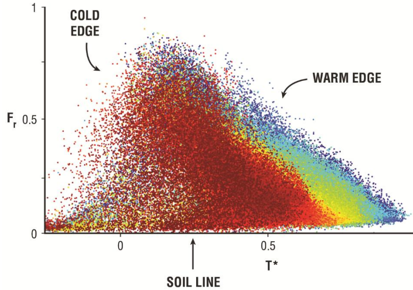
Figure 2. Triangle created from Sentinel-3 image made over Spain at 1 km resolution plotted as a scatterplot of fractional vegetation cover F_r versus T^* . Vertices A, B and C are referred to in the text, respectively, as NDVI_o/T_{max} , NDVI_s/T_{min} and NDVI_o/T_{min} . Salient features of the triangle are labeled. Colors represent pixel density, red being the most dense. Courtesy of George Petropoulos. Based on a figure from [20].
