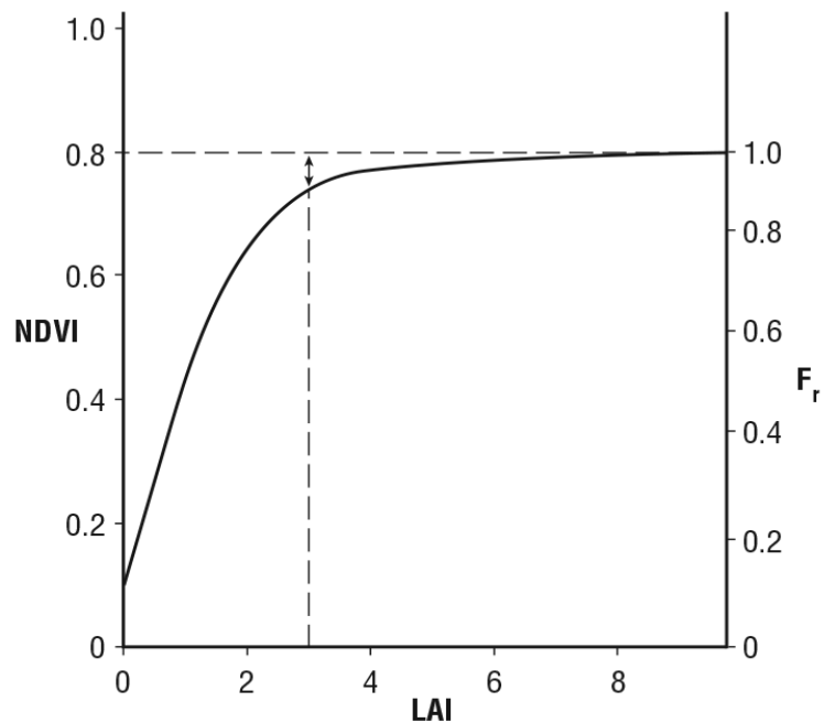
Figure 5. A representation of simulations with a land surface model of NDVI versus leaf area index (LAI), showing that full vegetation cover (NDVIs; F_r = 1 ), approximated by the horizontal dashed line at NDVI=0.8 , is obtainable for vegetation cover with an LAI larger than a value of about 3. Choice of NDVIs when LAI is near or below 3 will yield a trapezoidal shape as in the unshaded part of the triangle in Figure 4 (Based on simulations made by [31] and [9]).
