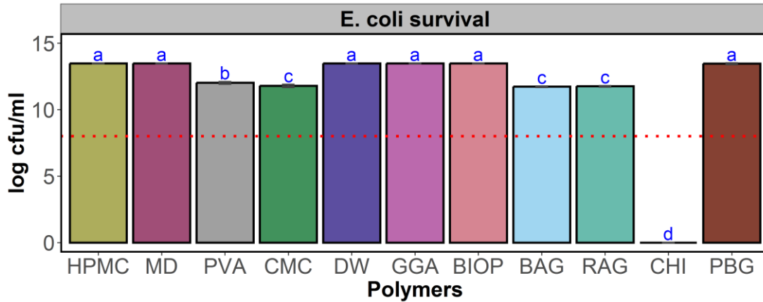
Fig. 3. Survival of E. coli cells in the polymer solutions. HPMC – hydroxypropyl methylcellulose; MD – maltodextrin; PVA – polyvinyl alcohol; CMC – carboxy methylcellulose; DW – dextrin white; GGA – guar gum; BIOP – biopolymer gel; BAG – brown algal gel; RAG – red algal gel; CHI – chitosan; PBG – phosphate buffer with glycerol. Each panel represents a mean of three replicates. The error bar indicates a standard error, and panels with different letters significantly differ (Tukey test, p < 0.01 ). In each panel, the red-dotted line indicates the optimum value of the trait based on the quality standard of liquid biofertilizer.
