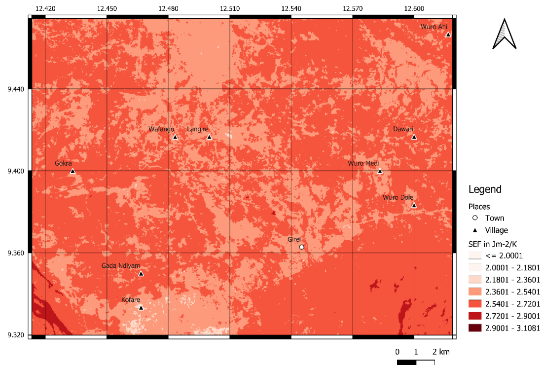
Figure 16: Wet Season (October) 2017 Surface Entropy Flux Map of Study Area ( \text{Jm}^{-2}\text{K}^{-1} )
