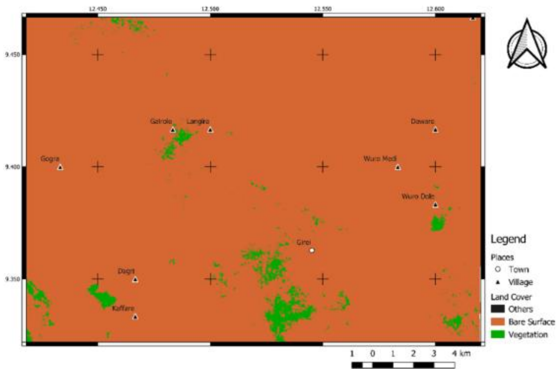
Figure 6: Vegetation Cover Map of Study Area for Dry Season (March) of 2015
