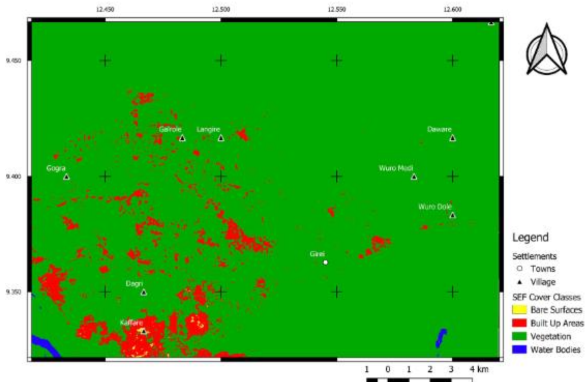
Figure 17: SEF Reclassified Land Cover Map of Study Area
