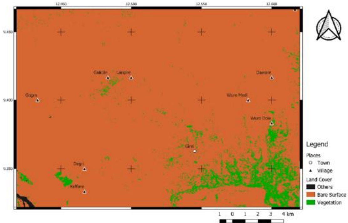
Figure 5: Vegetation Cover Map of Study Area for Dry Season (March) of 2013.
