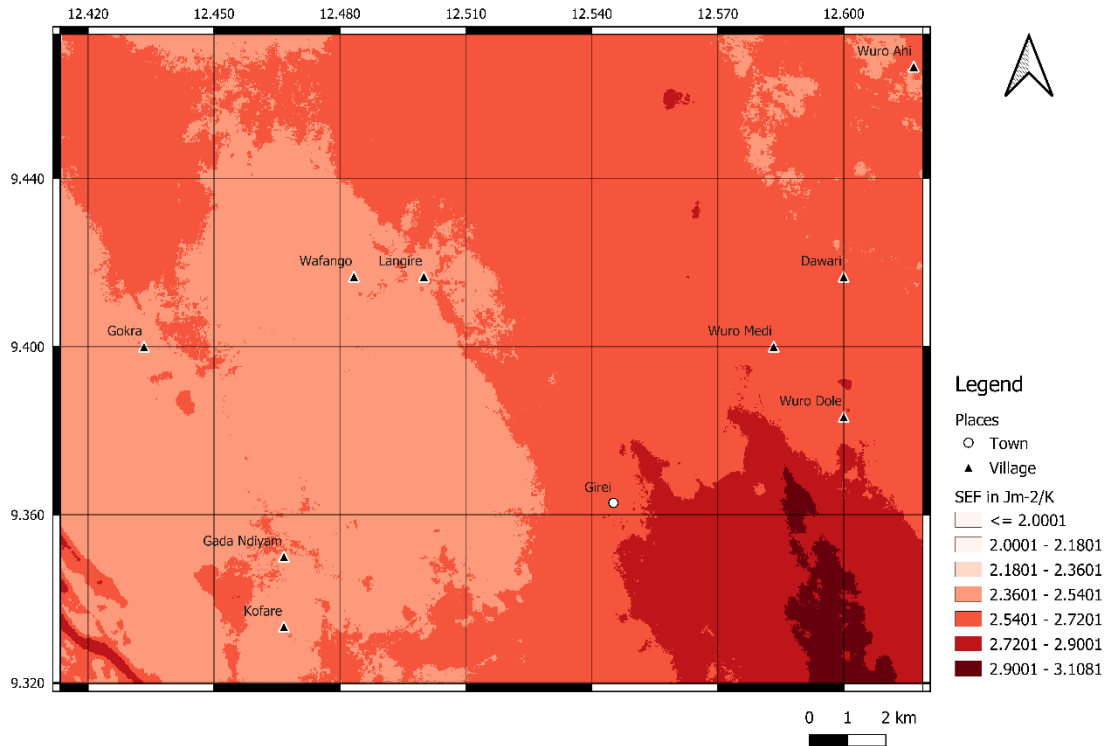
Figure 12: Dry Season (March) 2015 Surface Entropy Flux Map of Study Area ( \text{Jm}^{-2}\text{K}^{-1} )
