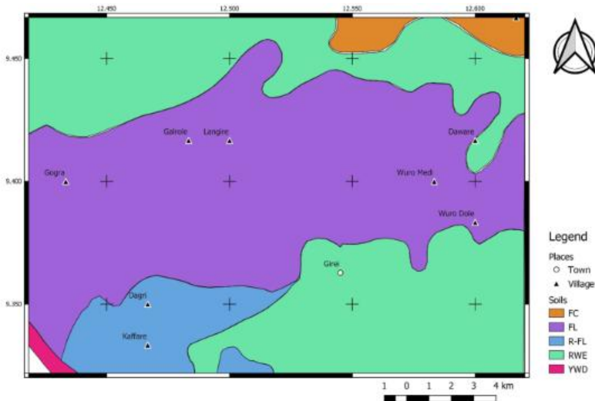
Figure 4: Soil Map of Study Area with Five Classes of Soils Overlaid with Towns and Villages
