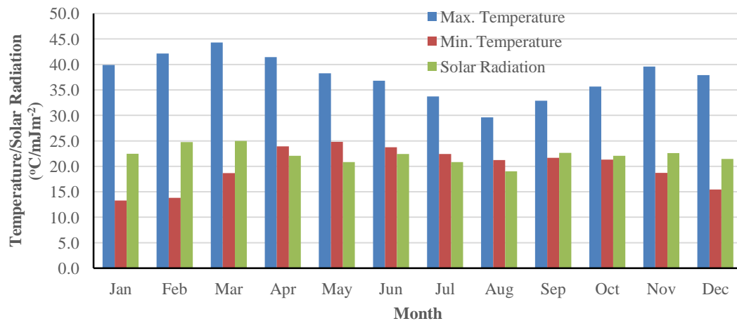
Figure 2: Monthly Averages of Temperature (Minimum and Maximum) and Solar Radiation
