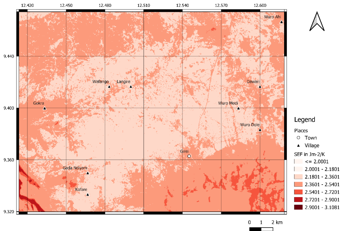
Figure 11: Dry Season (March) 2013 Surface Entropy Flux Map of Study Area ( \text{Jm}^{-2}\text{K}^{-1} )
