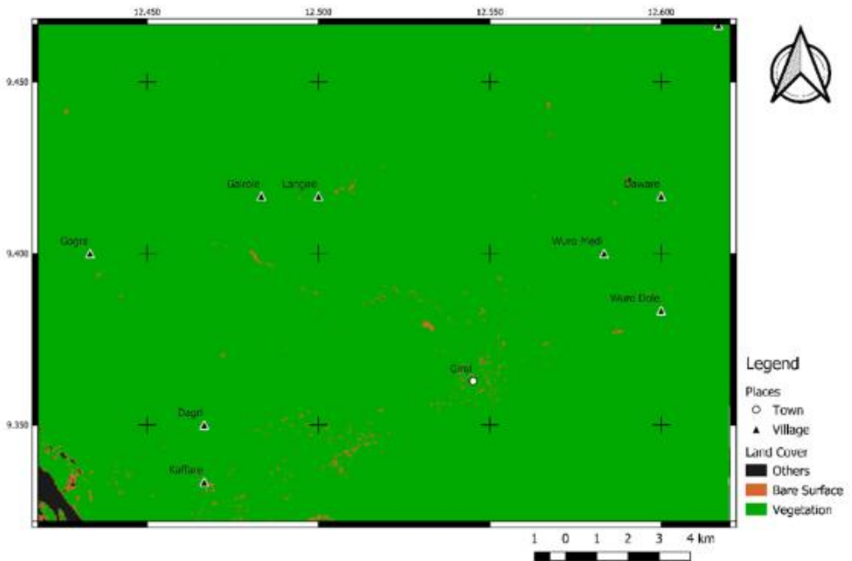
Figure 8: Vegetation Cover Map of Study Area for Wet Season (September) of 2013
