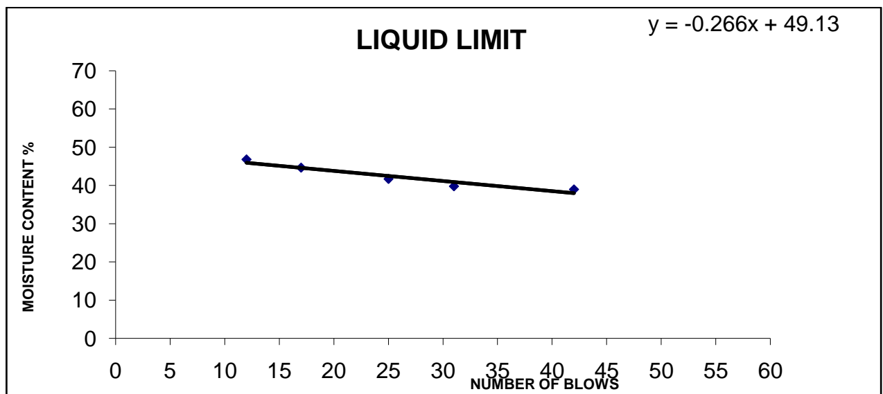
FIGURE 4: Graph of no of blows against moisture content for sample 2
