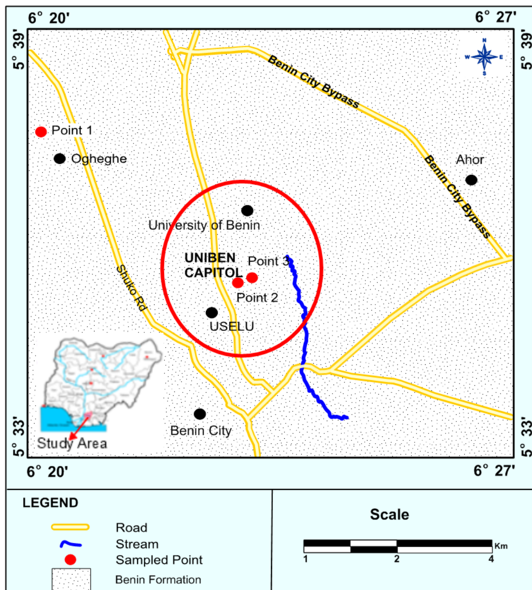
DIAGRAM 1: Map of the study area (Capitol gully)
