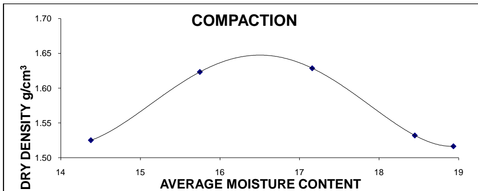
FIGURE 10: Graph of average moisture content against dry density for sample 2
