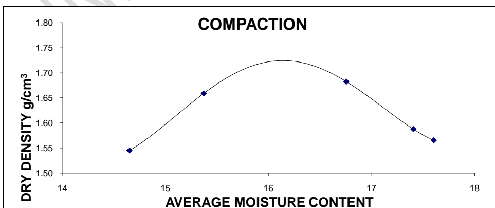
FIGURE 9: Graph of average moisture content against dry density for sample 2
