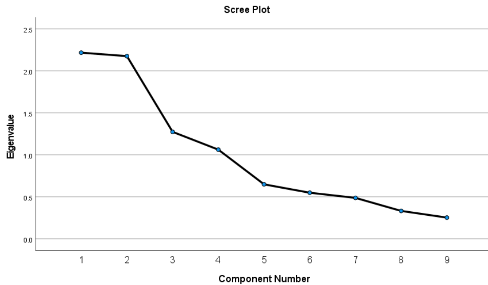
Fig 1 Scree plot
