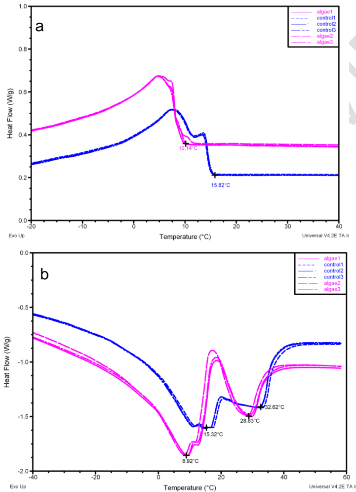
Fig. 2. Differential scanning calorimetry thermographs for the melting and crystallization of control and DHA enriched milk fat, immediately upon crystallization.
