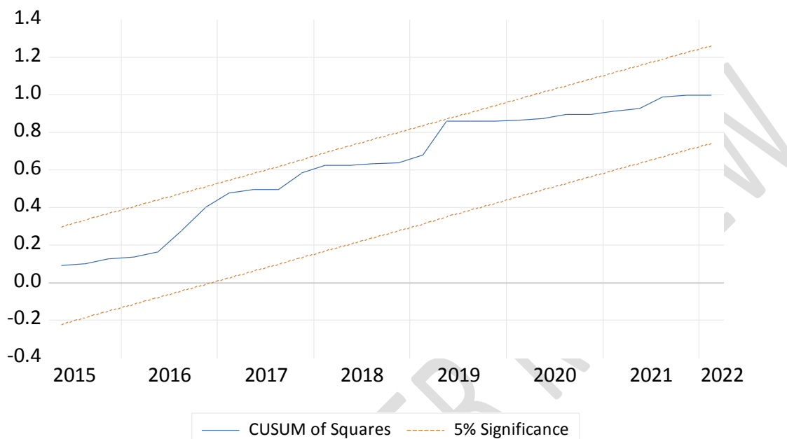
Fig 1 :Graphical presentation showing CUSUM of squares
