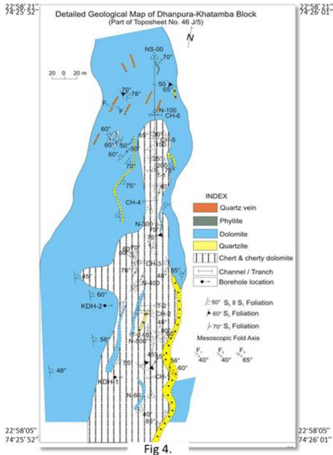
Fig 4. Detailed geological map of Dhanpura-Khatamba block, Jhabua District, M.P. Depicting disposition of chert in the area which is phosphatic in nature
