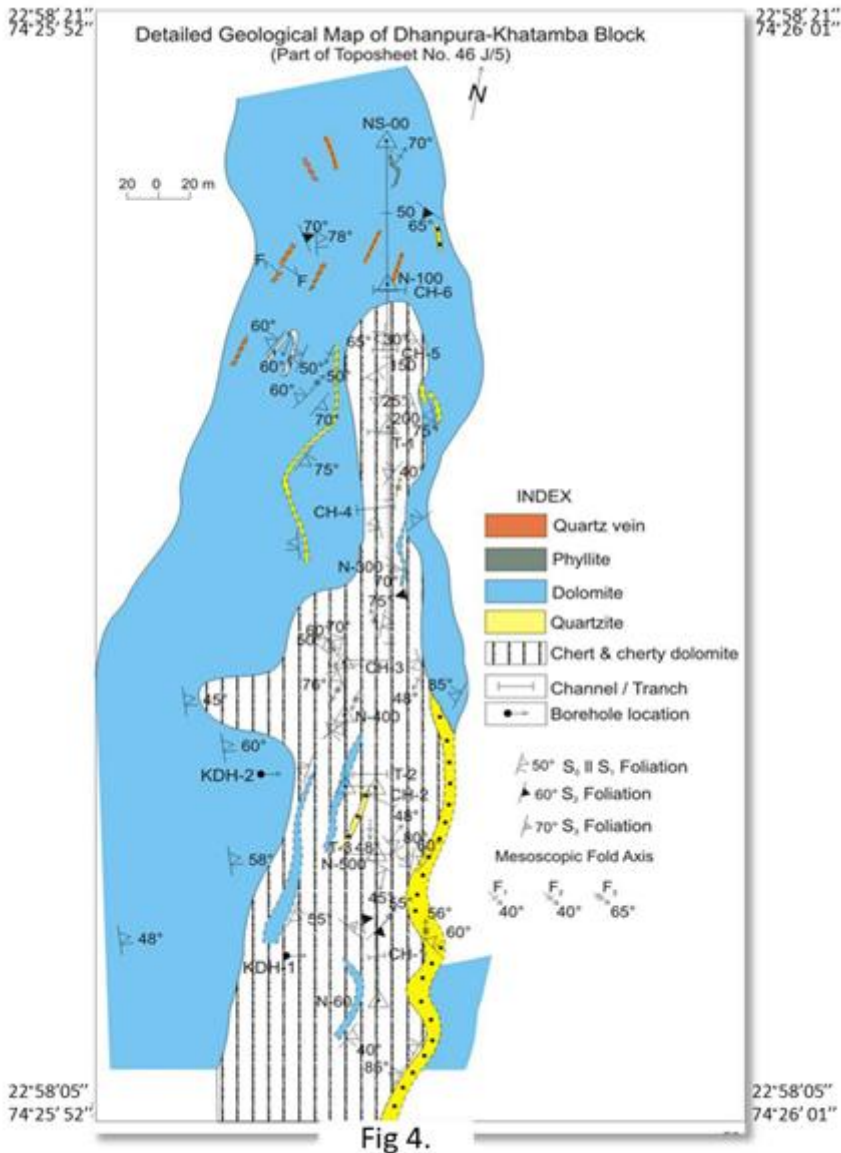
Fig 4. Detailed geological map of Dhanpura Khatama block, Jhabua District, M.P. Depicting disposition chert in the area which is phosphatic in nature
