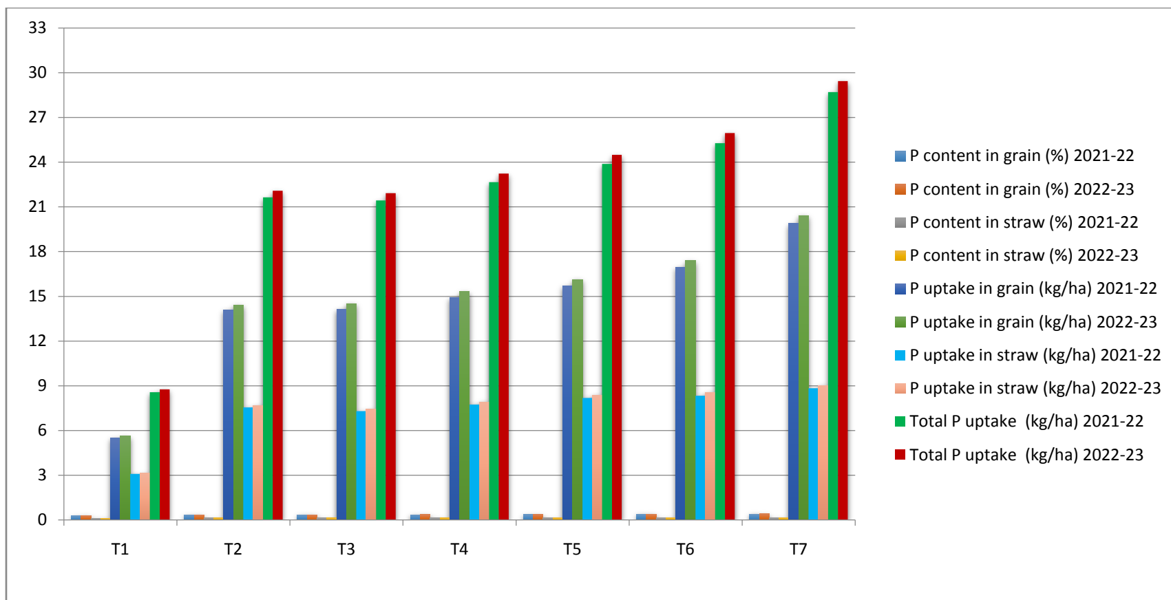
Fig. 2 Effect of different nutrient management approaches on P content (%), P uptake and Total P uptake (kg ha -1 ) in grain and straw of wheat
