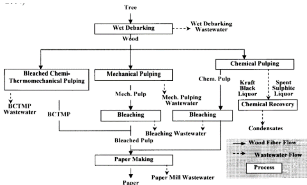
Figure 1. Different processes involved in pulp and paper production and corresponding
