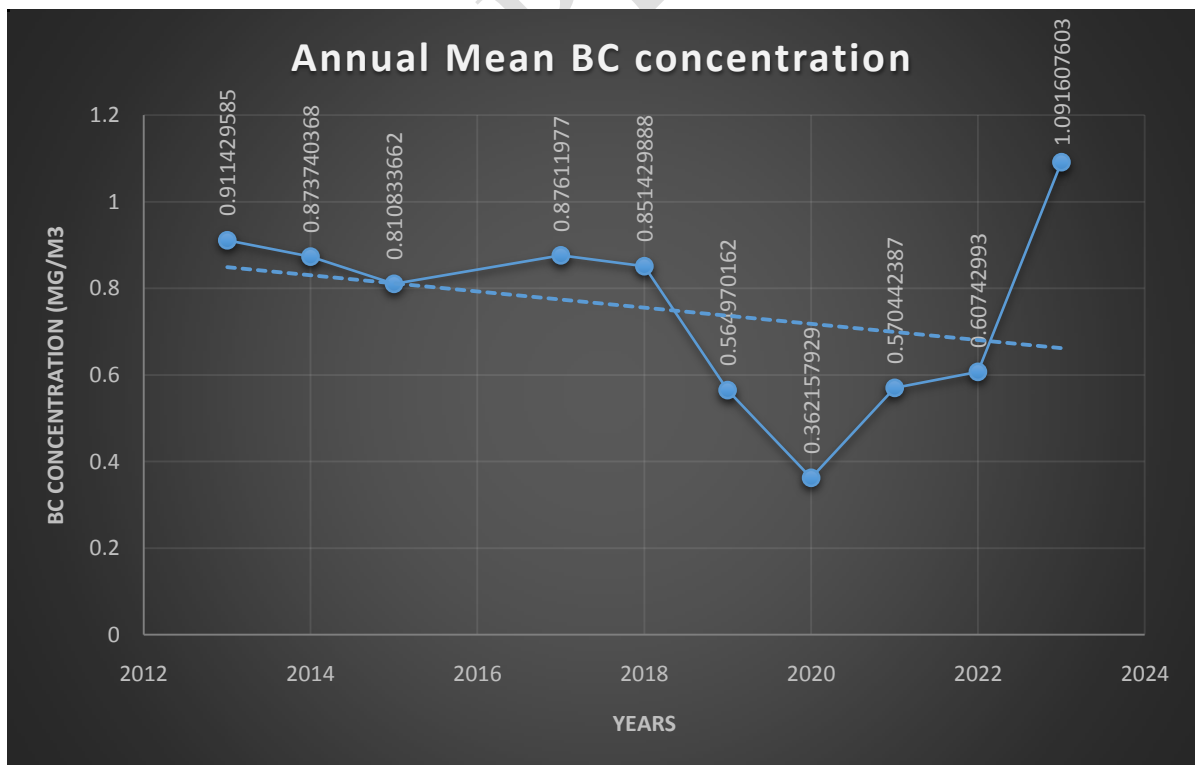
Figure.13. Annual Mean BC concentration (µg/m 3 ) during 2013 to 2023
