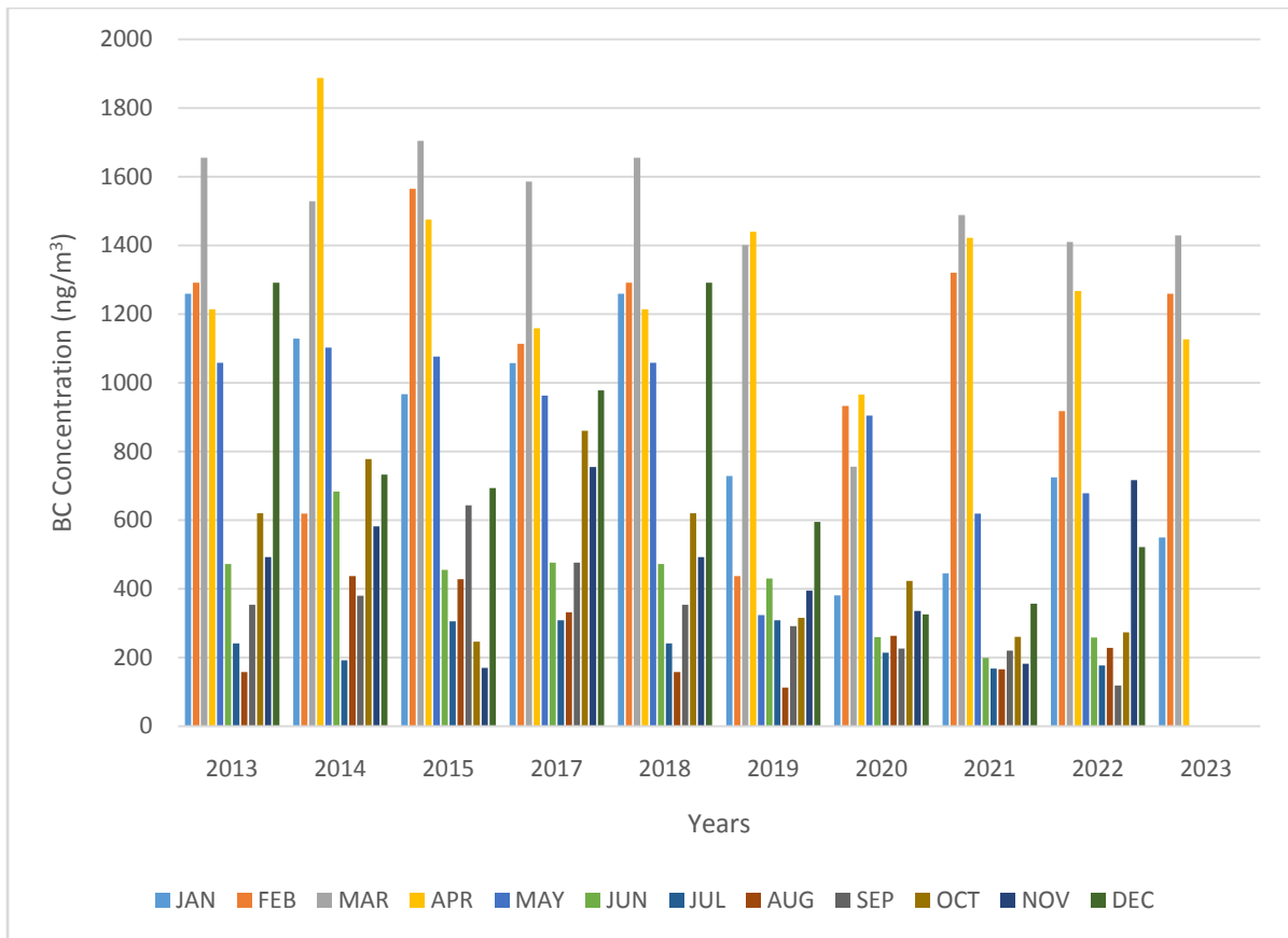
Figure.12. Monthly Mean BC (ng/m 3 ) concentration during different years
