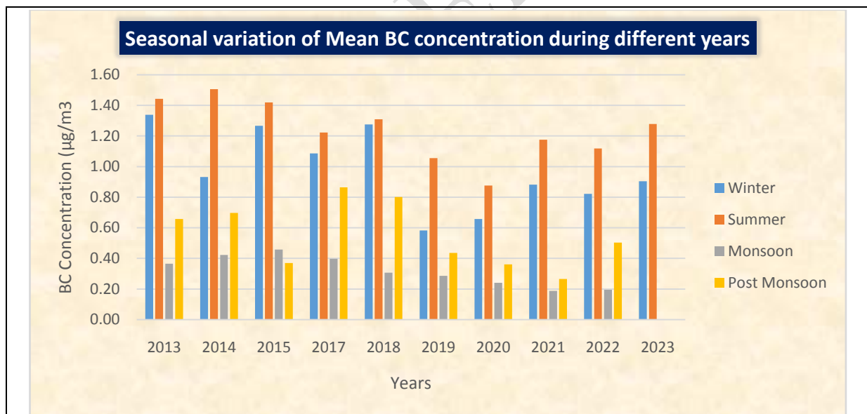
Fig .14. Overall seasonal variation of mean BC concentration ( \mu\text{g}/\text{m}^3 ) between 2013 and 2023
