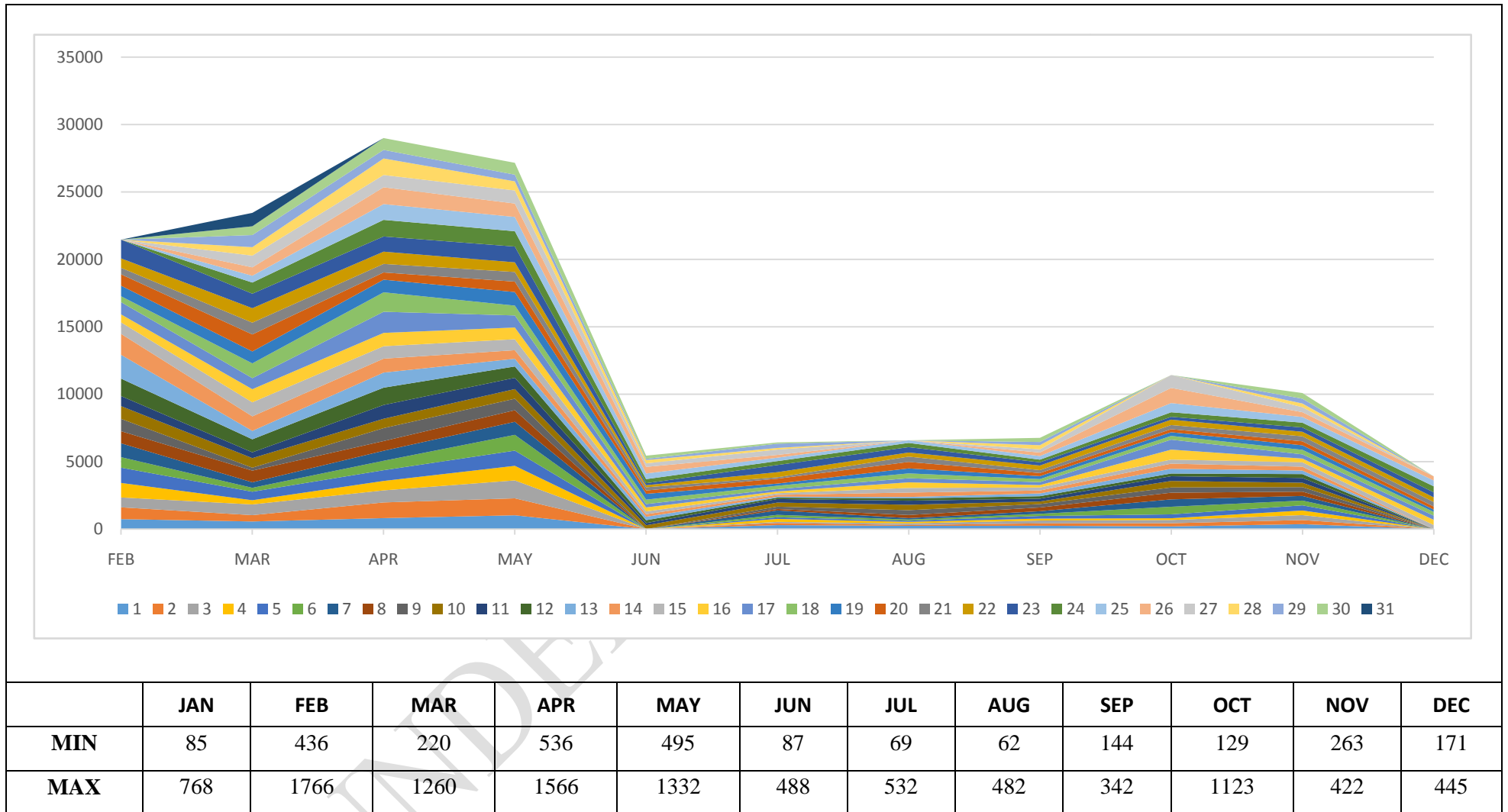
Figure.8. Temporal variations of monthly mean concentration (ng/m 3 ) during 2020
