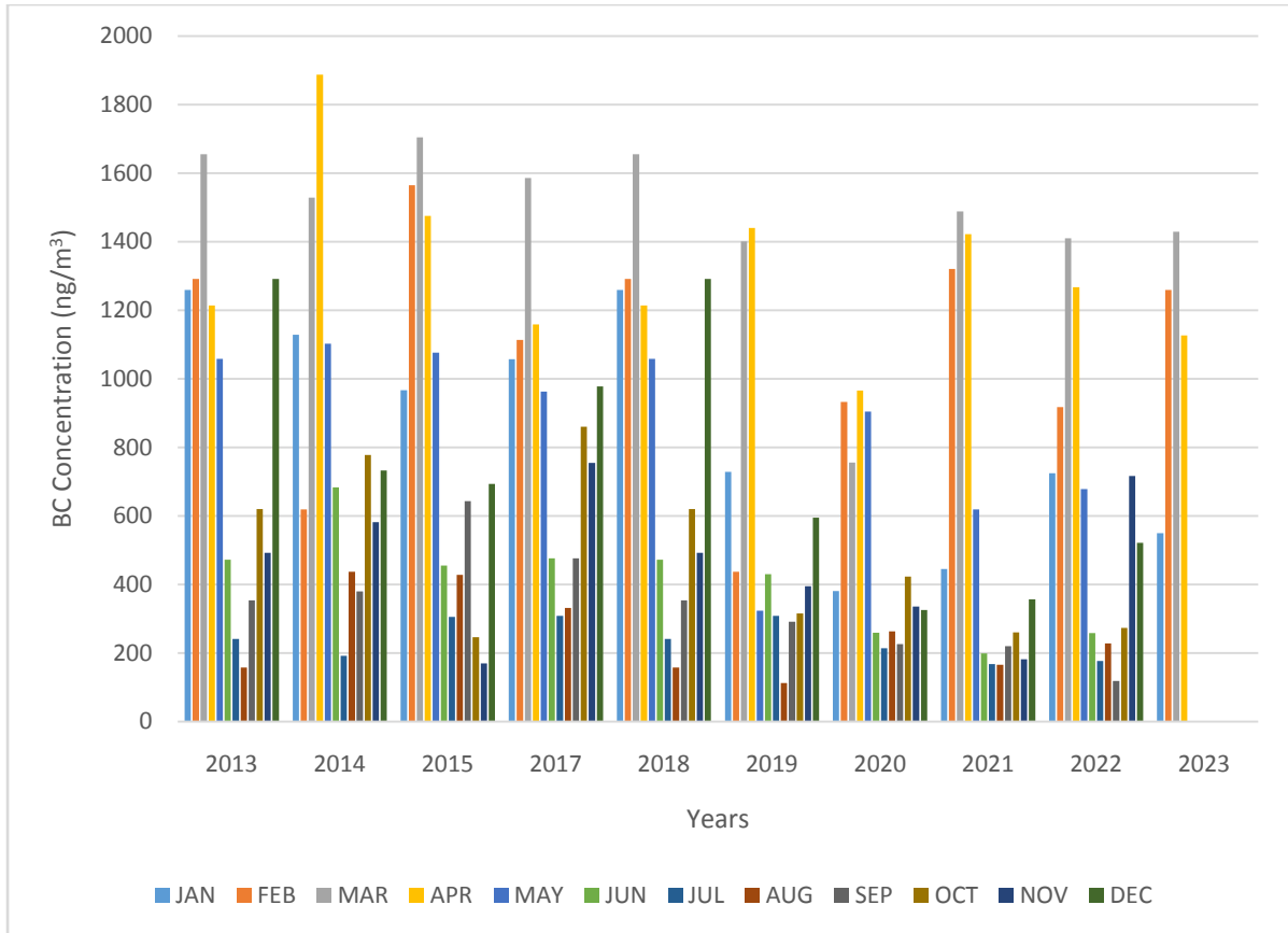
Figure.12. Monthly Mean BC ( \text{ng/m}^3 ) concentration during different years
