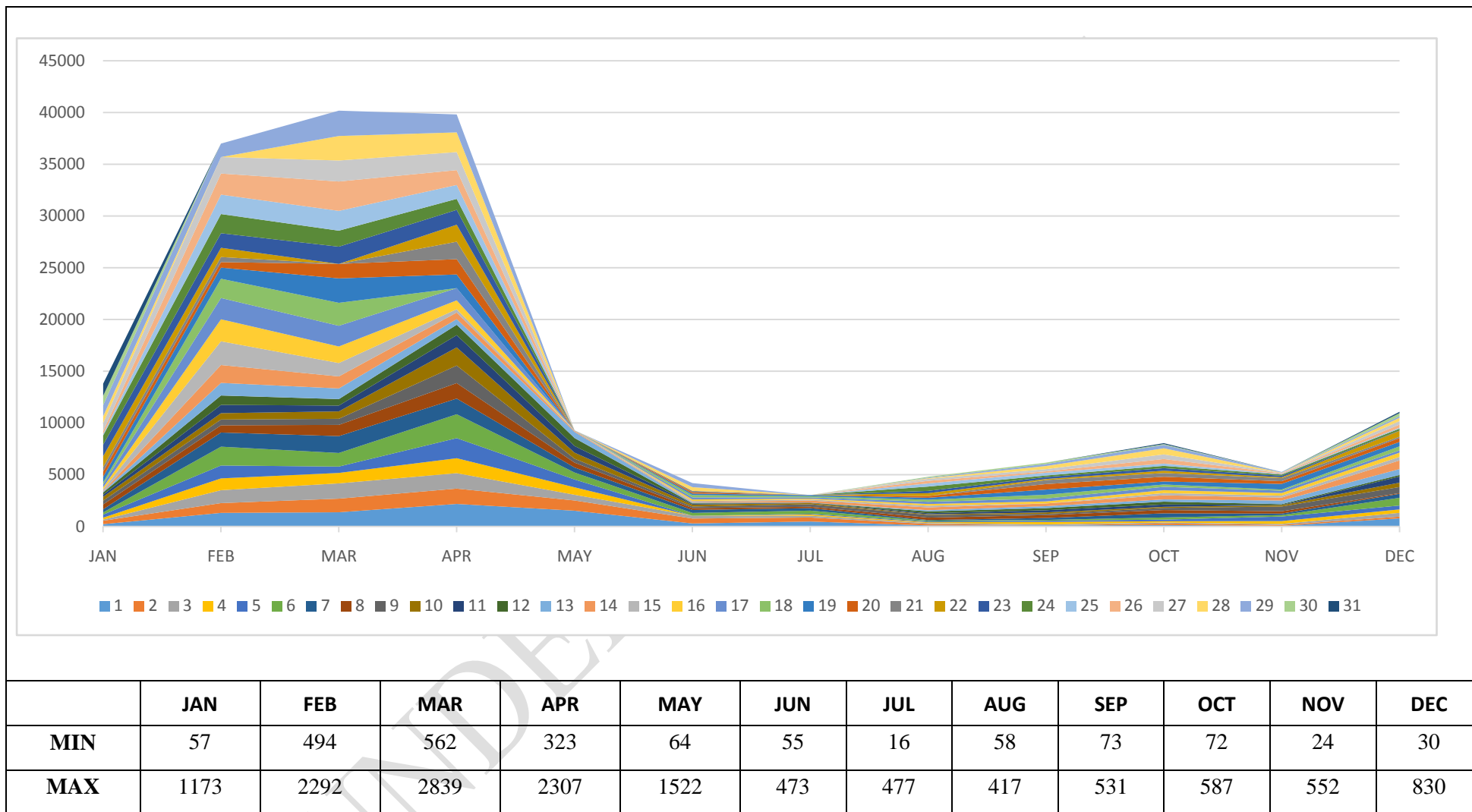
Figure.9. Temporal variations of monthly mean concentration (ng/m 3 ) during 2021
