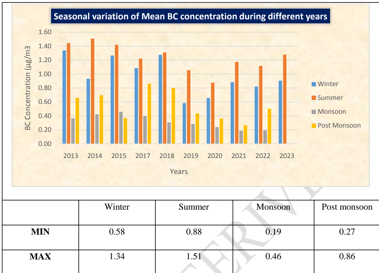
Fig .15. Seasonal variation of mean BC concentration ( \mu\text{g}/\text{m}^3 ) between 2013 and 2023
