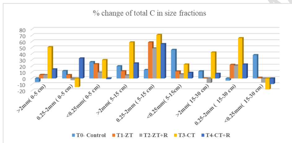
Fig 2: % change of total carbon in aggregate size fractions due to influence of tillage and crop residue management in long-term experimental plot observed between Post-Wheat soil 2018 and Post-Rice 2019
