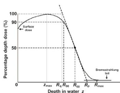
Figure 1 Typical electron beam PDD curve of R_q , R_p , R_{max} , R_{50} and R_{90} (Podgorsak, 2003).
