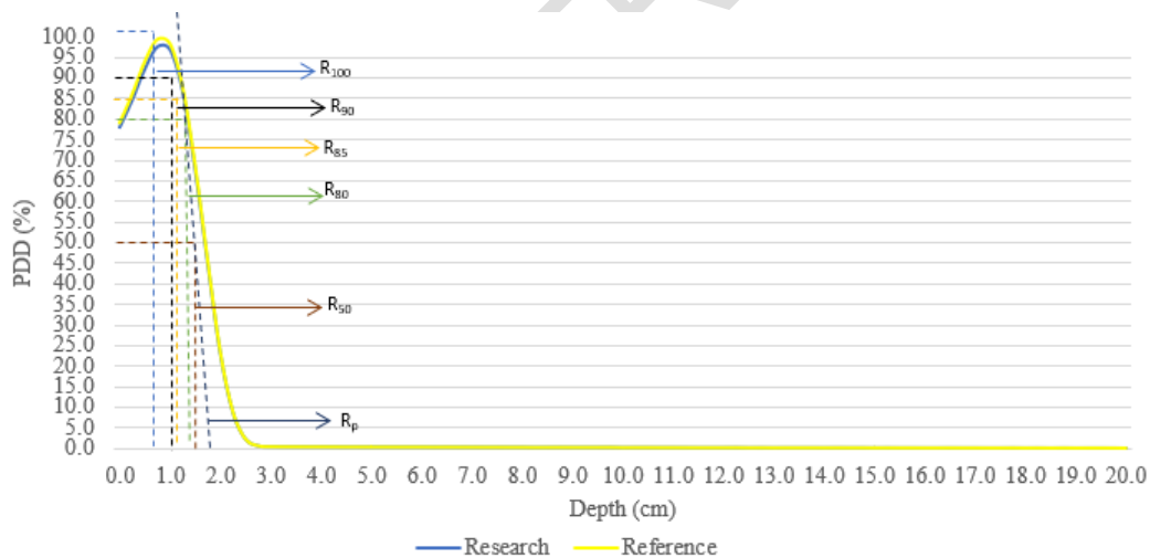
Figure 2 Graph of measurement results of R_{100} , R_{90} , R_{85} , R_{80} , R_{50} , and R_p and with the values set by AAPM to 4 MeV energy.
