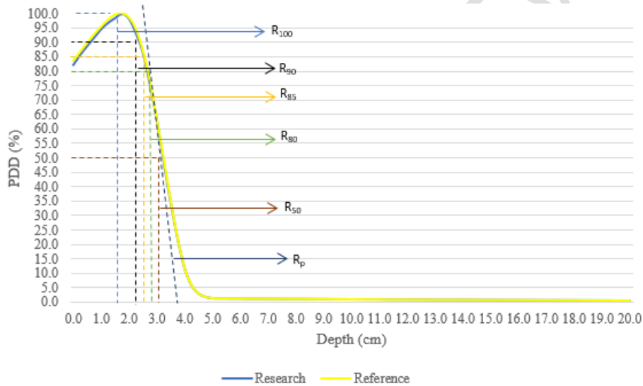
Figure 4 Graph of measurement results of R_{100} , R_{90} , R_{85} , R_{80} , R_{50} , and R_p and with the values set by AAPM to 8 MeV energy.
