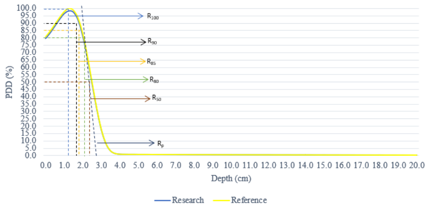
Figure3 Graph of measurement results of R_{100} , R_{90} , R_{85} , R_{80} , R_{50} , and R_p and references to 6 MeV energy.
