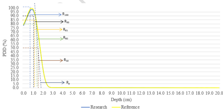
Figure 2 Graph of measurement results of R_{100} , R_{90} , R_{85} , R_{80} , R_{50} , and R_p and references to 4 MeV energy.
