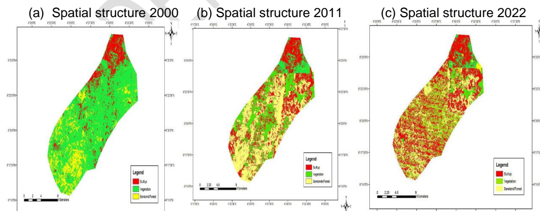
Fig. 2: Spatial structure of Eyenkorin in 2000, 2011 and 2022
