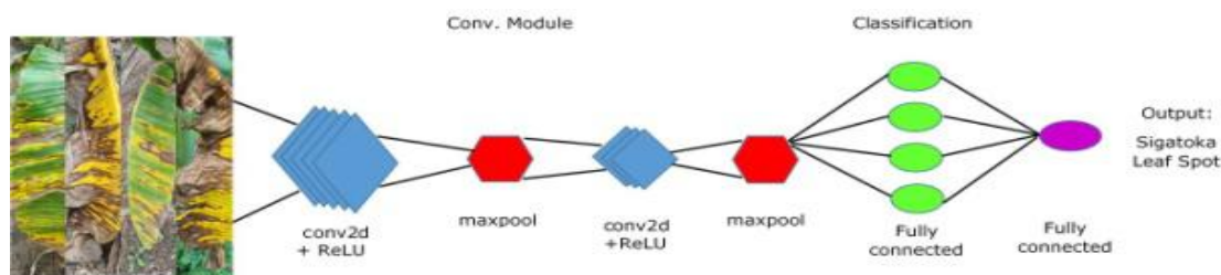
Fig. 3. CNN architecture for banana disease diagnosis
