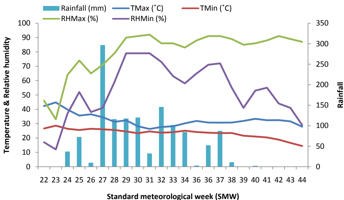
Fig. 1 Meteorological observations during crop growth season
