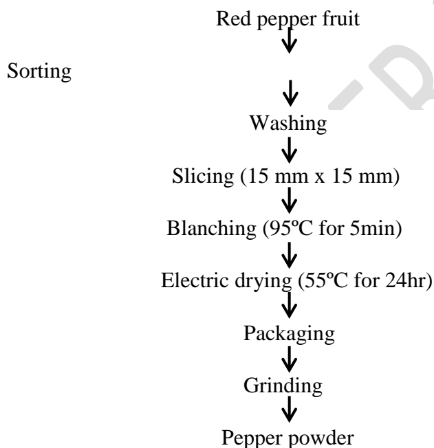
Fig. 1: Flow chart for pepper powder preparation.
