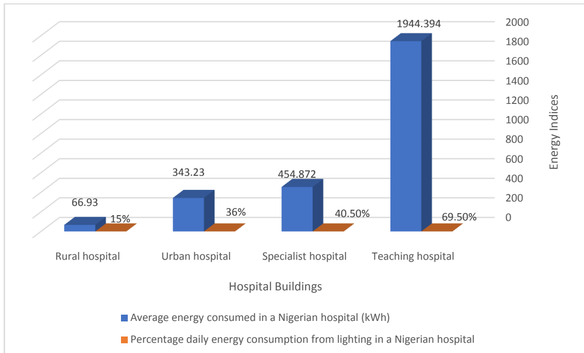
Figure 1: Energy performance indices for hospital buildings in Nigeria.
