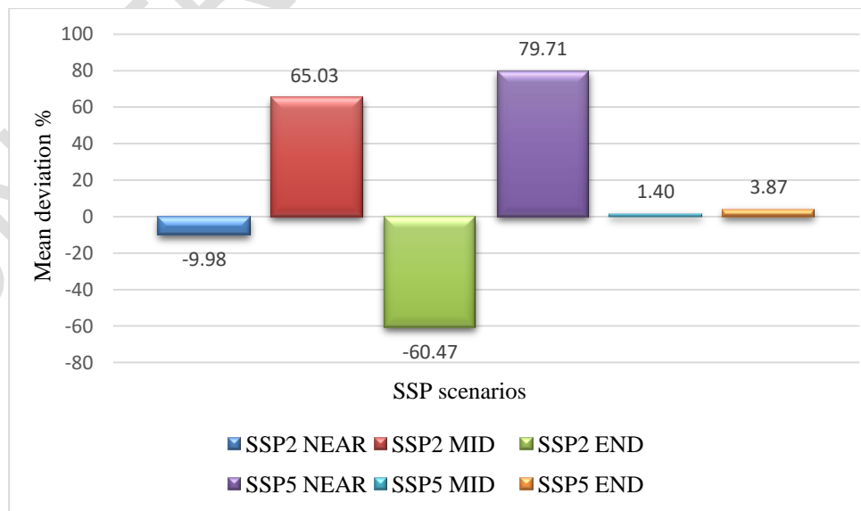
Fig 7. NEM precipitation percentage of Mean deviation in Tamil Nadu region
