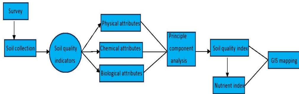
Fig. 1. Flow diagram of methodology of the study
