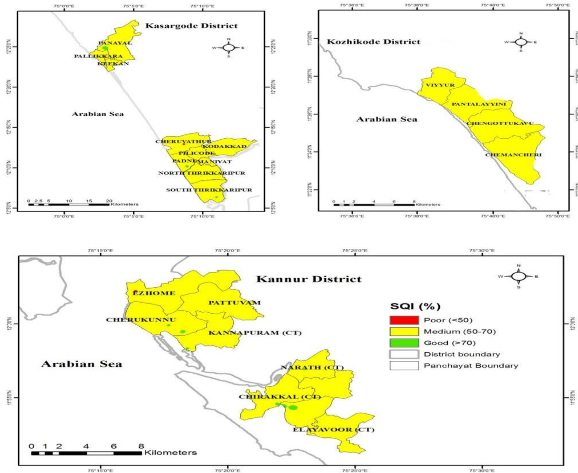
Fig. 5. Spatial variability of SQI in AEU 7
