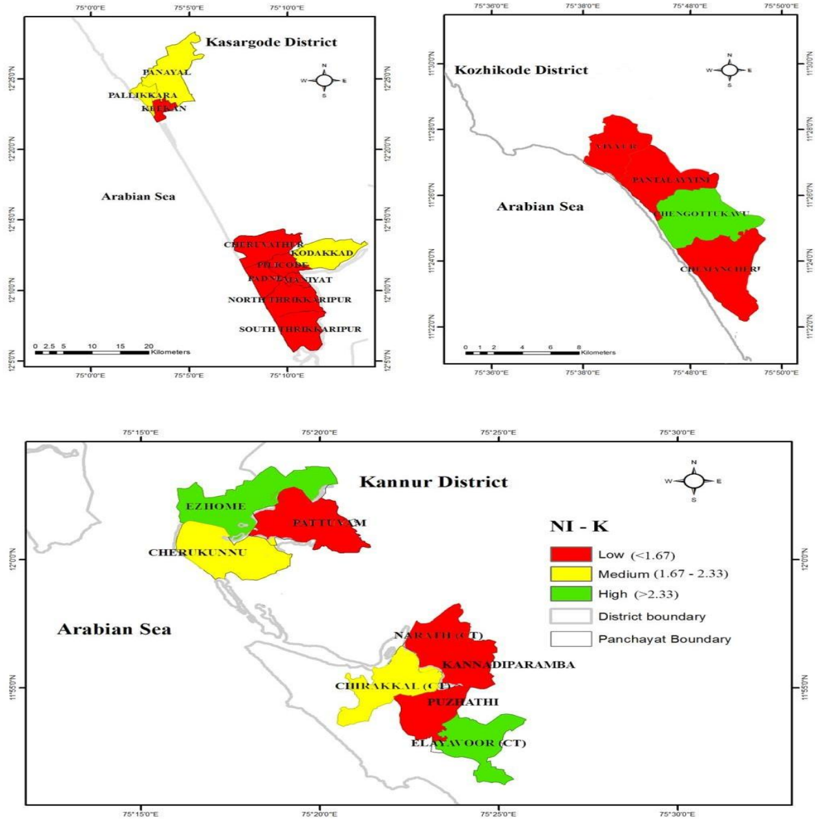
Fig. 8. Spatial variability of NI of available K in AEU 7
