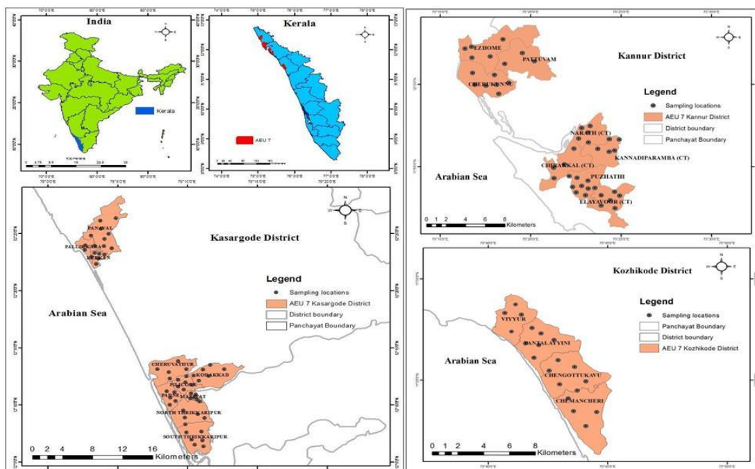
Fig. 2. Location map of study area and sampling sites in (a) Kannur, (b) Kasargode and (c) Kozhikode districts of Kaipad (AEU 7)
