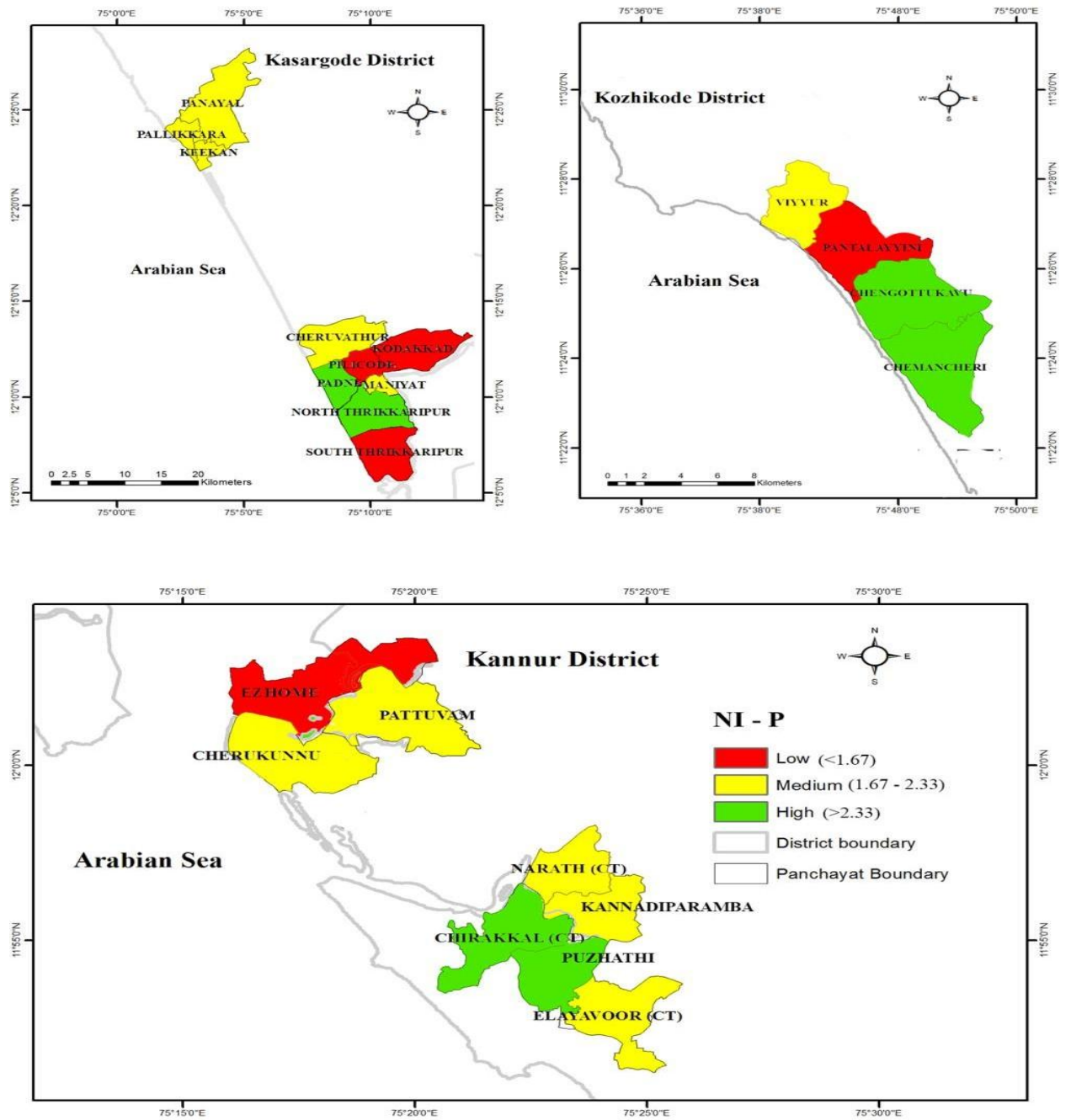
Fig. 7. Spatial variability of NI of available P in AEU 7
