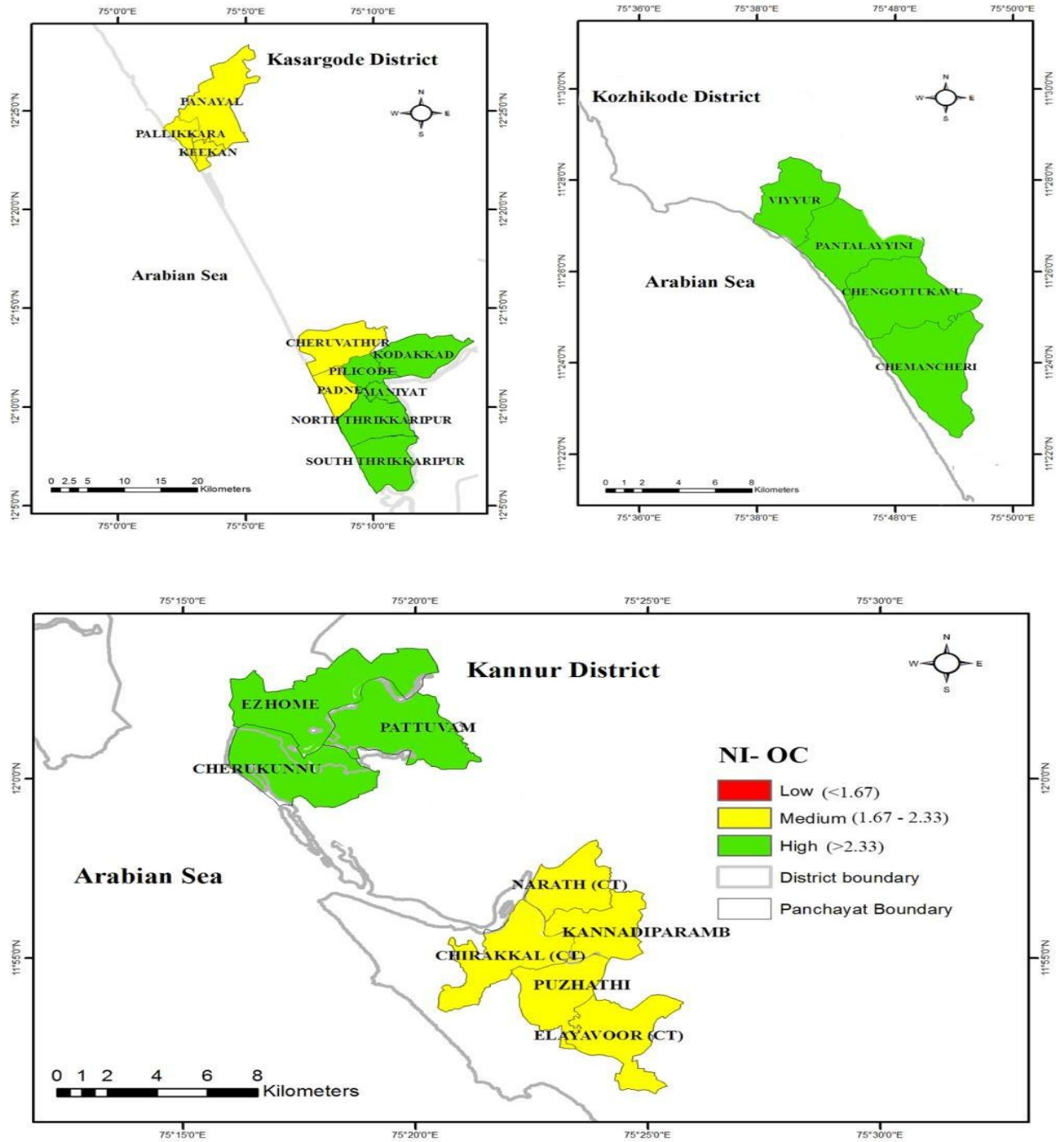
Fig. 6. Spatial variability of NI of organic carbon in AEU 7
