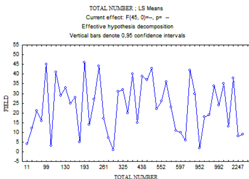
Figure 3 : Mean number of spores per field
