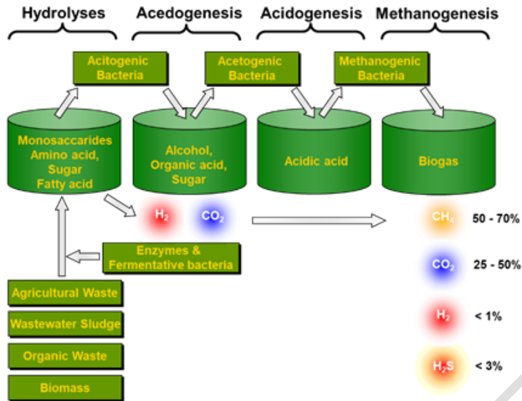
Figure 1: Pathway of anaerobic digestion by Dölle et. al. [8].
