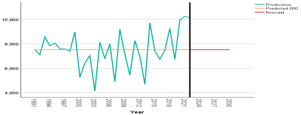
Fig 4. Forecasting groundnut Production in India using ARIMA (0,0,0)
