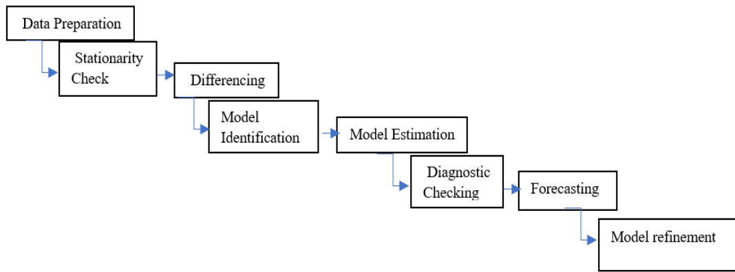
Chart 1. Procedure flow chart of ARIMA modelling and forecast (Source: Author's own compilation)
