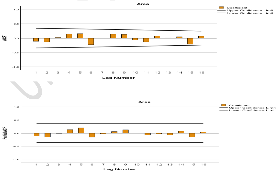
Fig 7. ACF and PACF plots of first differenced data of groundnut area in Telangana
