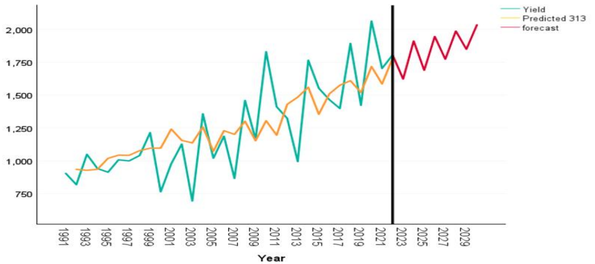
Fig 6. Forecasting groundnut Yield in India using ARIMA (3,1,3)
