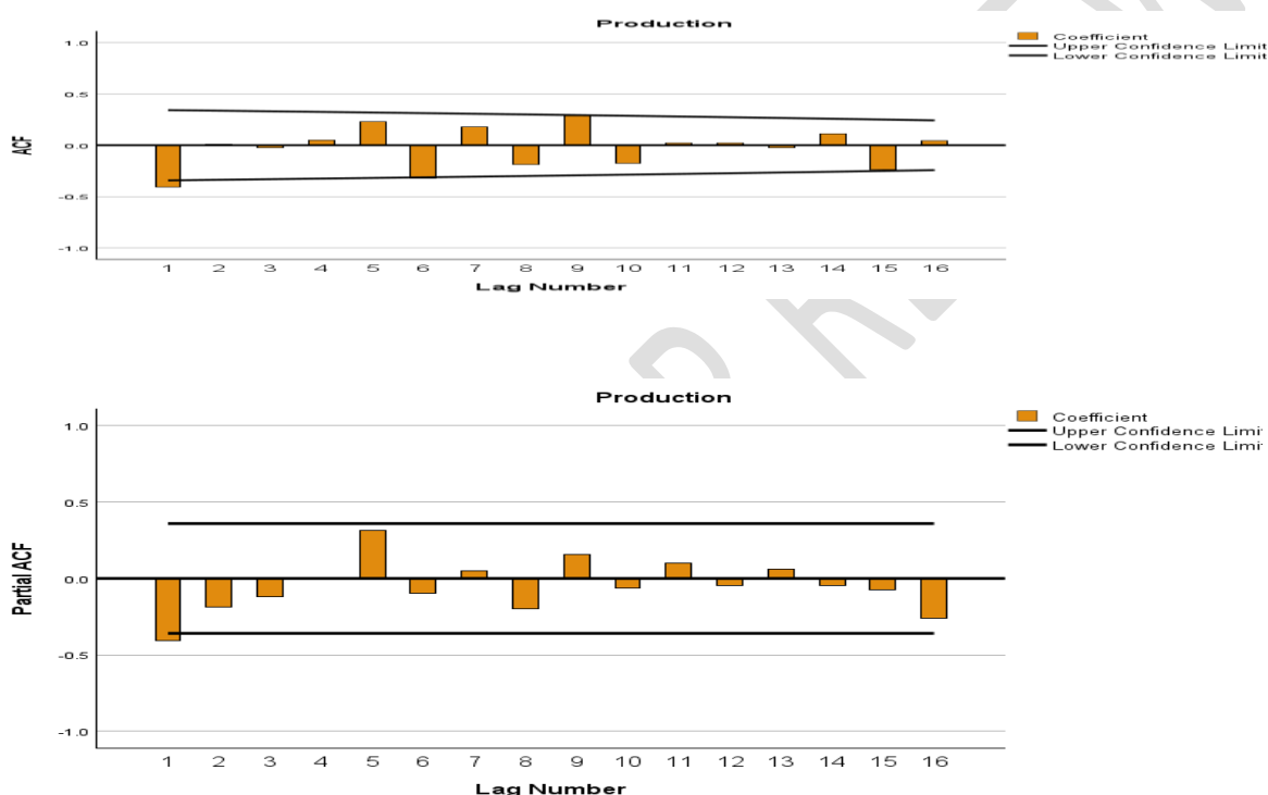
Fig 9. ACF and PACF plots of level data of groundnut production in Telangana
