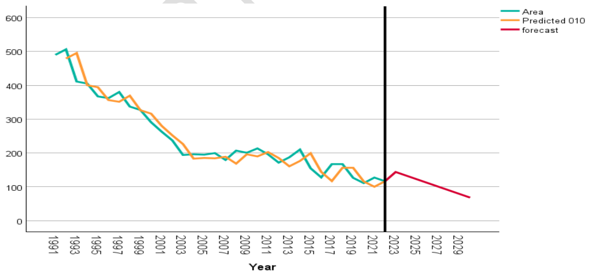
Fig 8. Forecasting groundnut area in Telangana using ARIMA (0, 1, 0)
