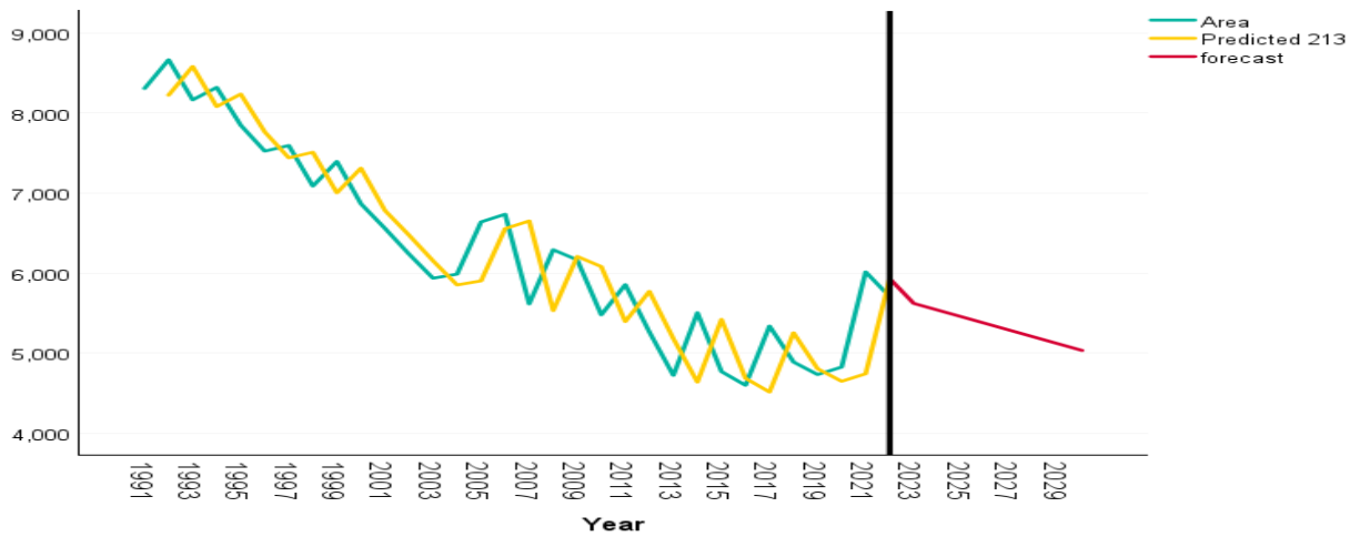
Fig 2. Forecasting groundnut area in India using ARIMA (2,1,3)
