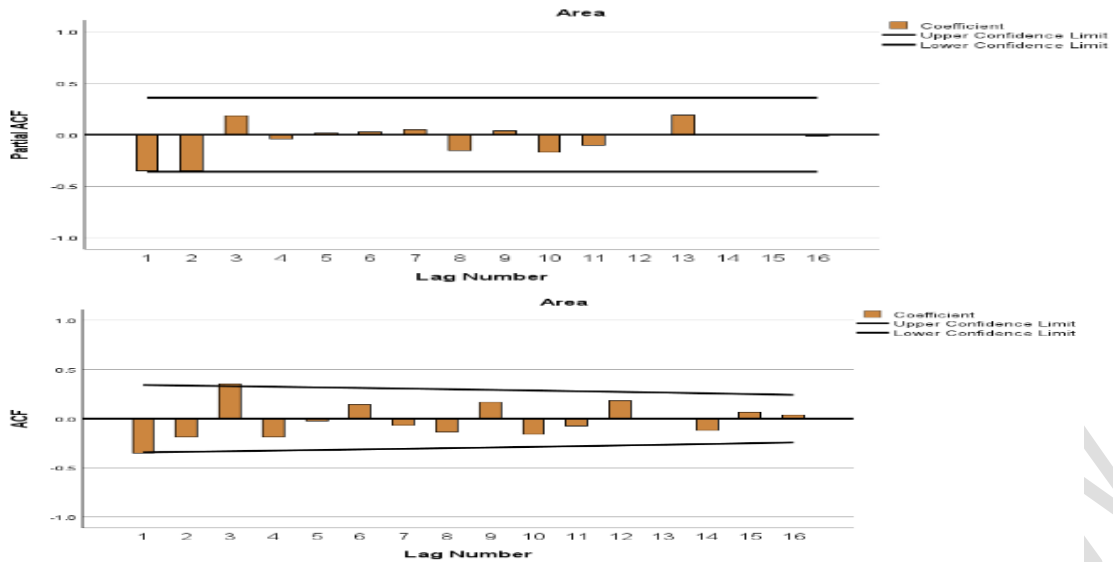
Fig 1. ACF and PACF plots of first differenced data of groundnut area in India
