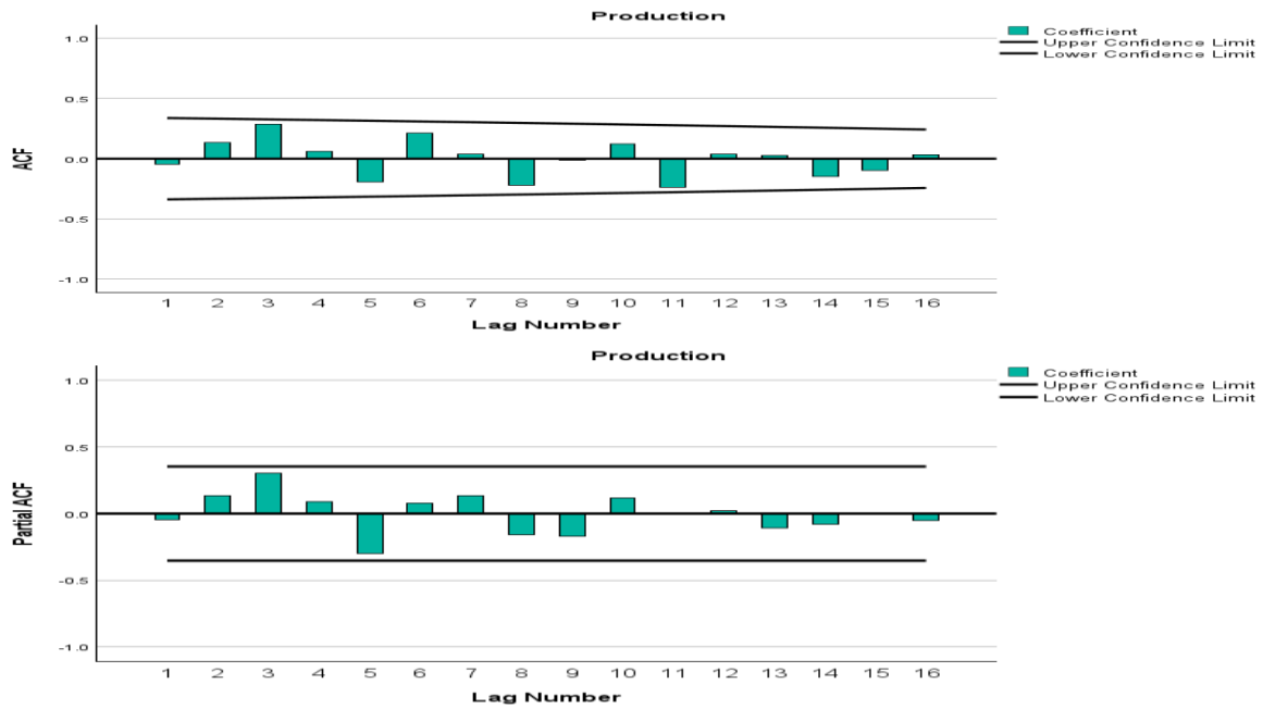
Fig 3. ACF and PACF plots of level data of groundnut Production in India
