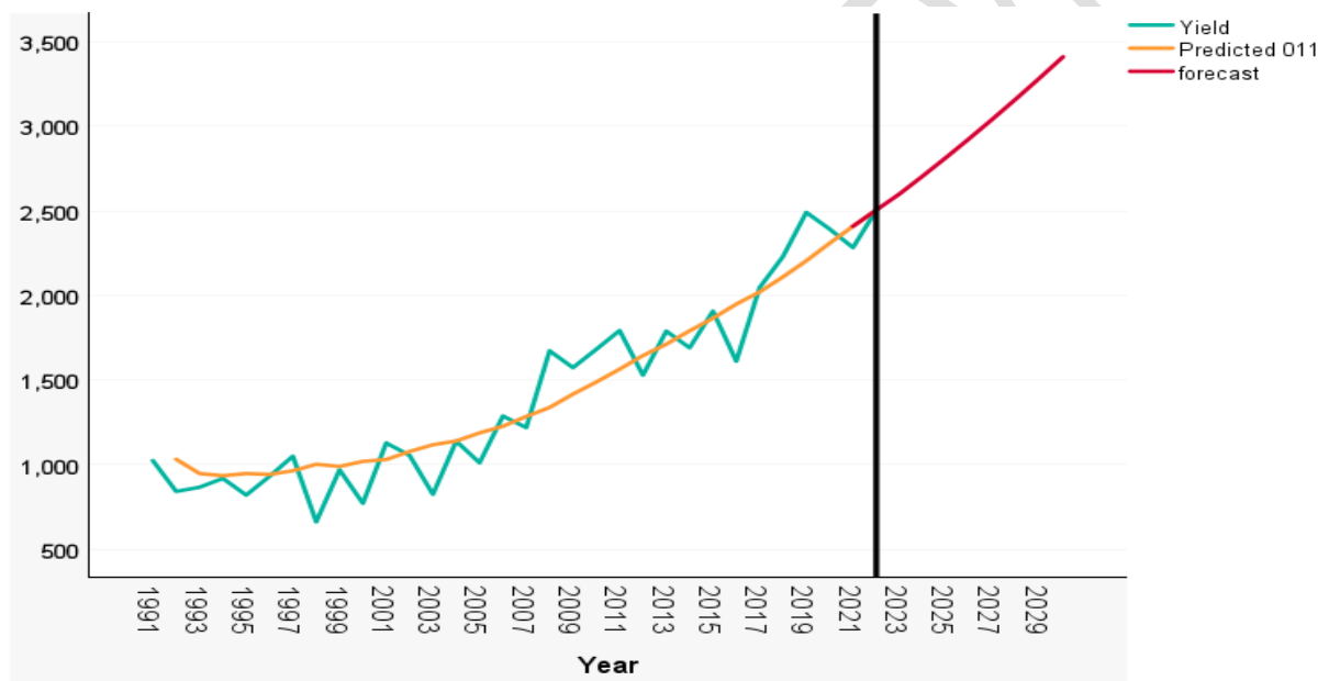
Figure 12. Forecasting groundnut yield in Telangana using ARIMA (011)
