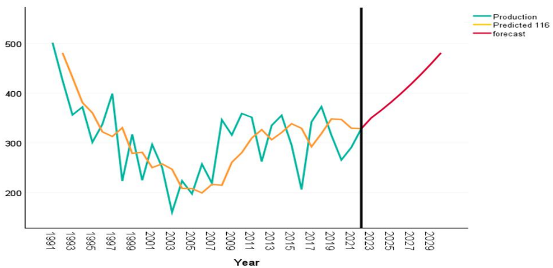
Fig 10. Forecasting groundnut production in Telangana using ARIMA (1, 1, 6)
