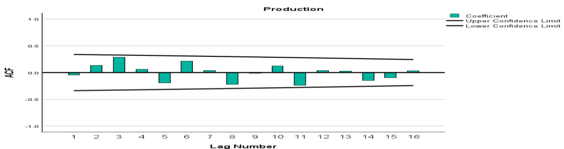
Fig 3. ACF and PACF plots of level data of groundnut Production in India
