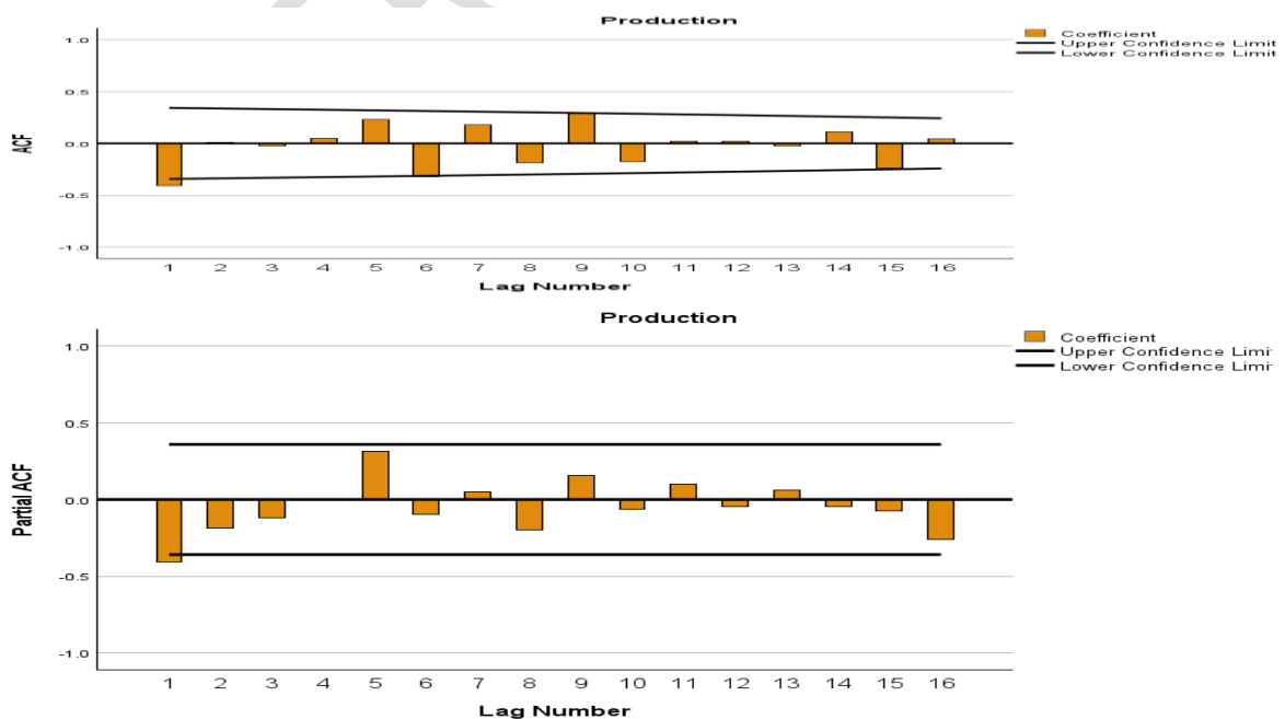
Fig 9. ACF and PACF plots of level data of groundnut production in Telangana
