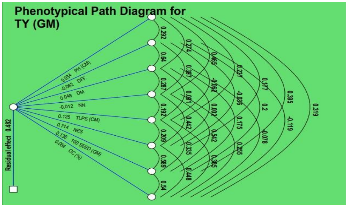
Fig. 2. Phenotypical path diagram of various traits with seed yield per plot in castor.
