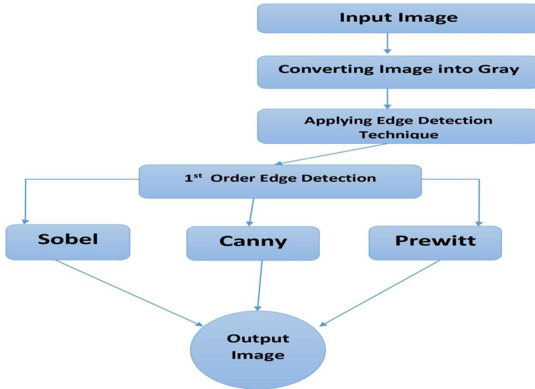
Figure 5. Flow Chart of Methodology
