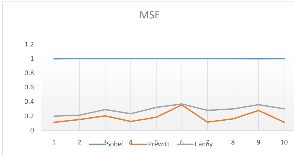
Figure 11. MSE graph of Sobel, Prewitt and Canny(Standard Images)
