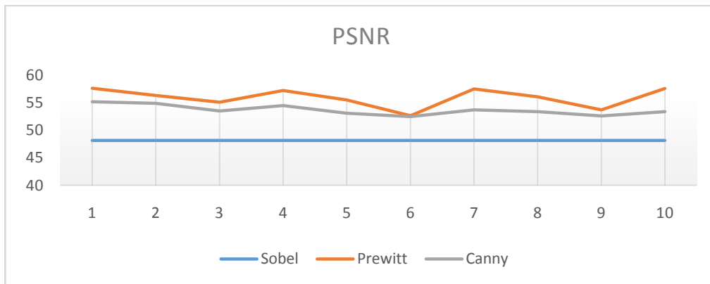
Figure 9. PSNR graph of Sobel, Prewitt and Canny (Standard Images)
