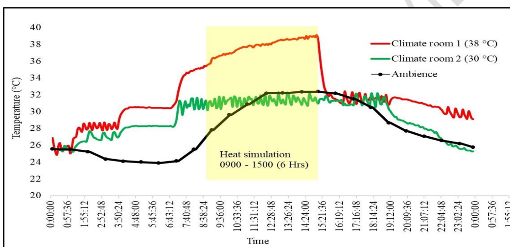
Fig. 1. Mean diurnal temperature variation inside climate-controlled rooms (30 and 38 °C) and ambience conditions under a rain shelter
