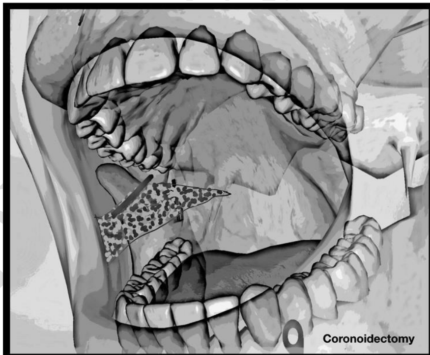
Fig 4. Coronoidectomy
