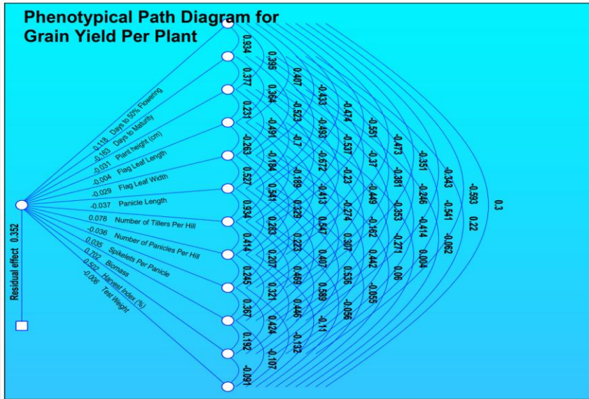
Fig. 2. Phenotypical Path Diagram
