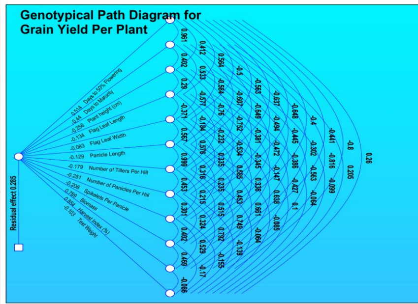
Fig. 3. Genotypical Path Diagram
