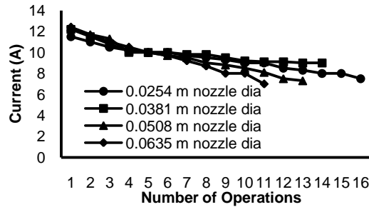
Fig. 17: Variation of Current with Number of Operations.
