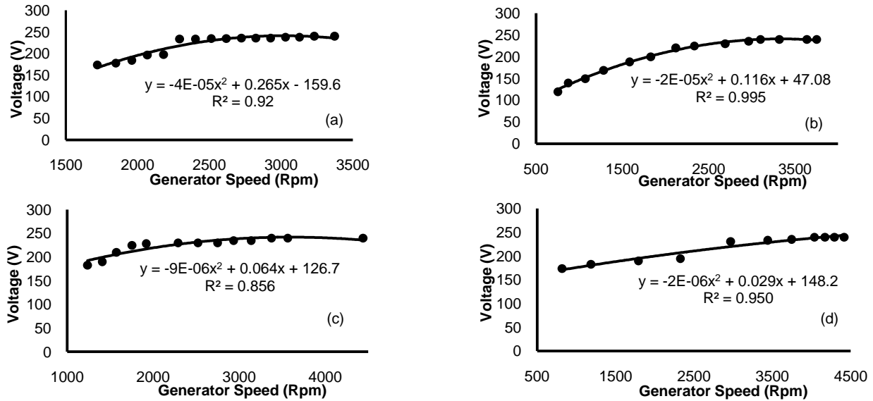
Fig. 19: Variation of Voltage developed with the Generator Speed for the (a) 0.0254 m, (b) 0.0381 m, (c) 0.0508 m and (d) 0.0635 m diameter Nozzles.
