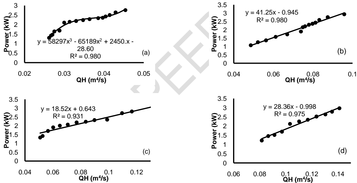
Fig. 20: Variation of Power developed with the Flow Rate – Head product for the (a) 0.0254 m, (b) 0.0381 m, (c) 0.0508 m and (d) 0.0635 m diameter Nozzles
