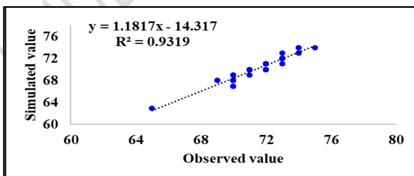
Fig.4. Comparison of observed and simulated values of days to anthesis of maize for 2018-19
