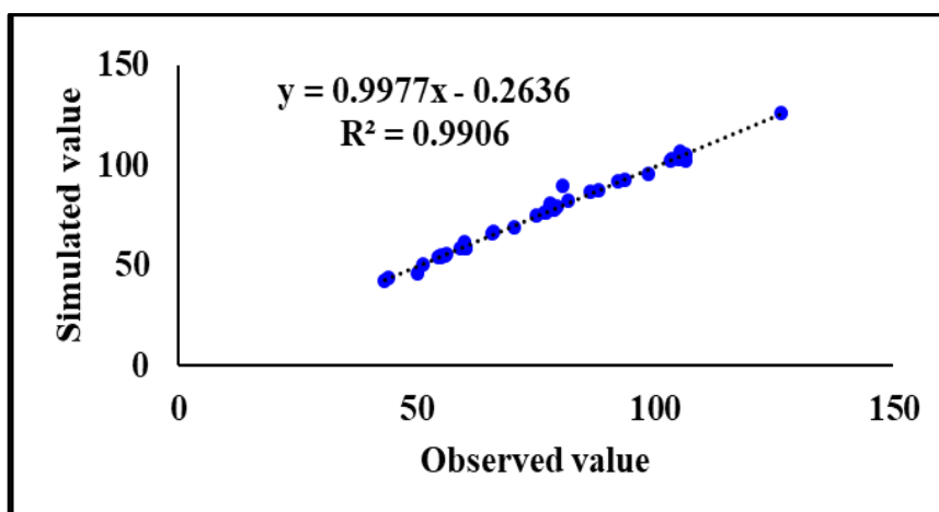
Fig.7. Comparison of observed and simulated maize grain yield in 2018-19 (calibration)
