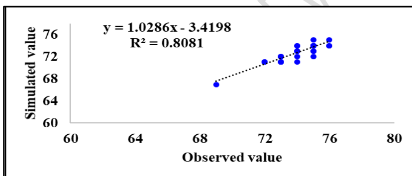
Fig.3. Comparison of observed and simulated values of days to anthesis of maize for 2018-19
