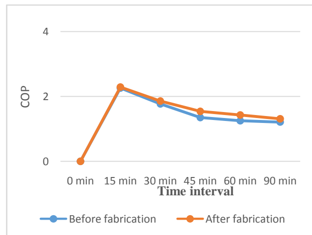
Fig 6 : Time vs. COP (comparison between data's of before fabrication and after fabrication)
