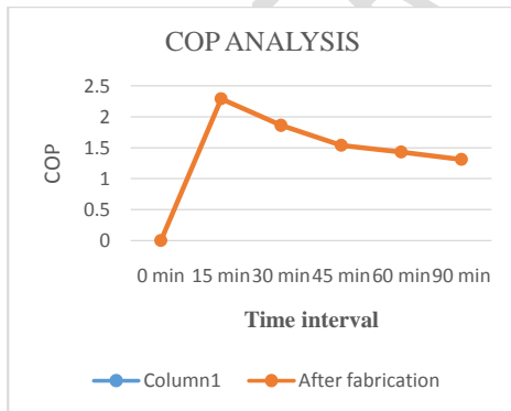
Fig 5: Time vs cop (After fabrication)
