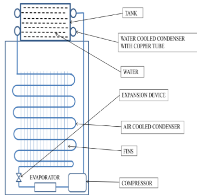
Fig 3: Line diagram of modified refrigerator
