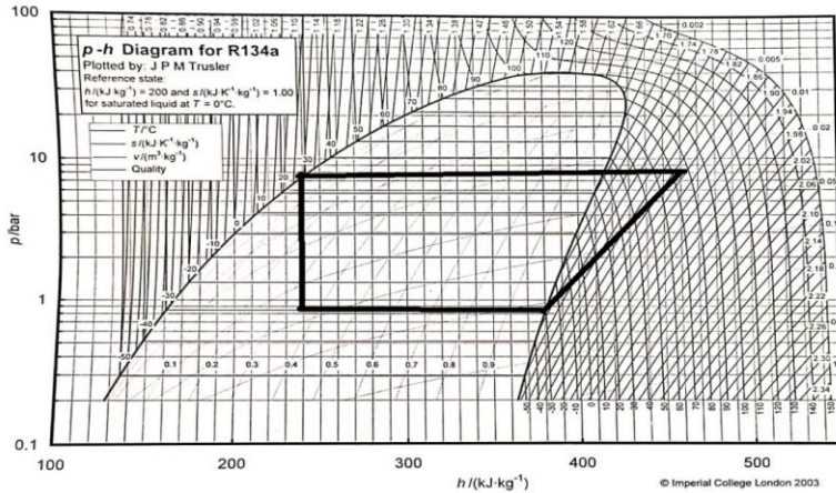
Fig 7: p-h diagram
