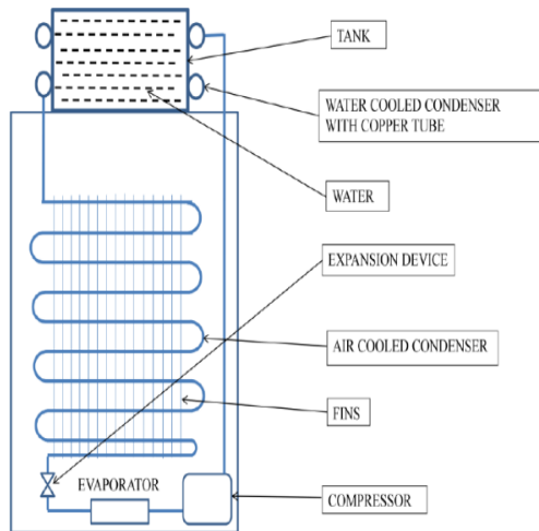
Fig 3: Line diagram of modified refrigerator
