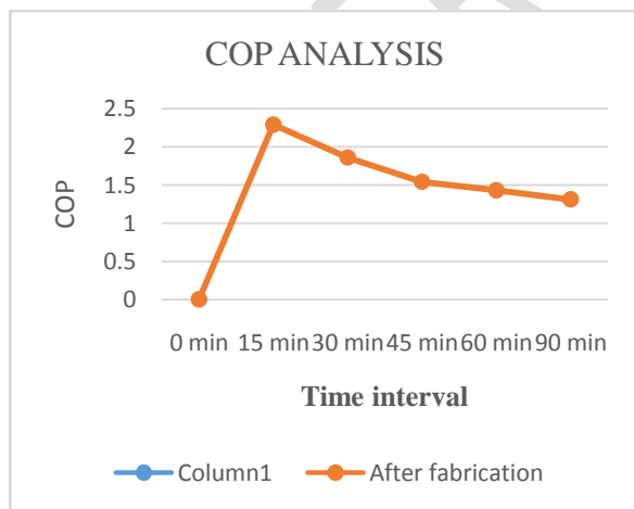
Fig 5: Time vs cop (After fabrication)
