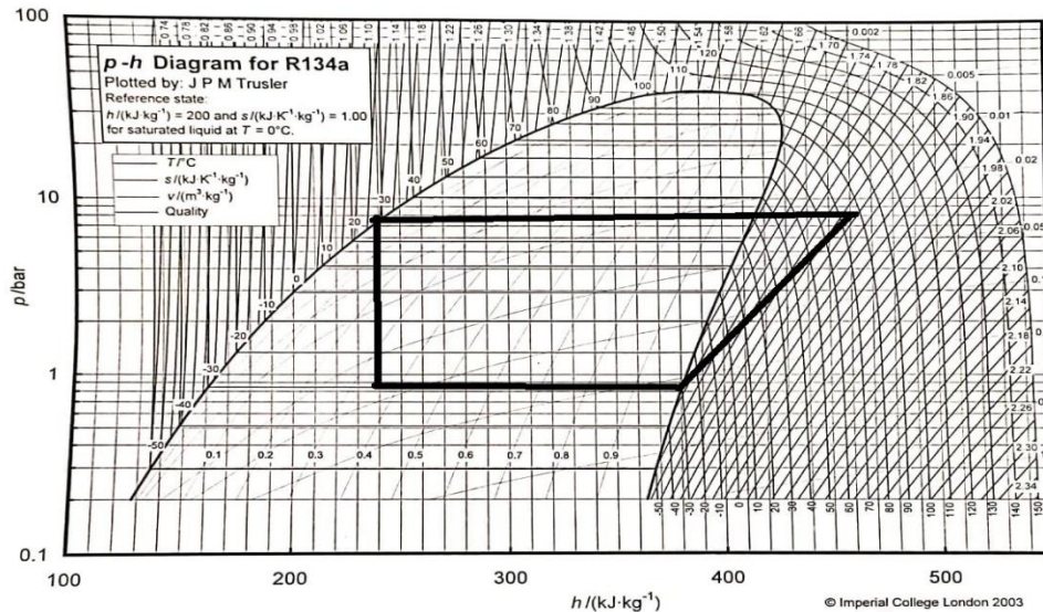
Fig 7: p-h diagram
