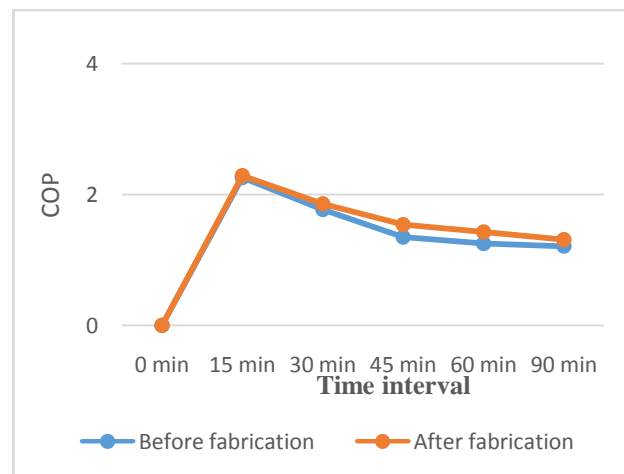
Fig 6 : Time vs. COP (comparison between data's of before fabrication and after fabrication)
