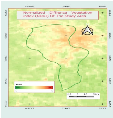
Fig.2 NDVI of the Area
