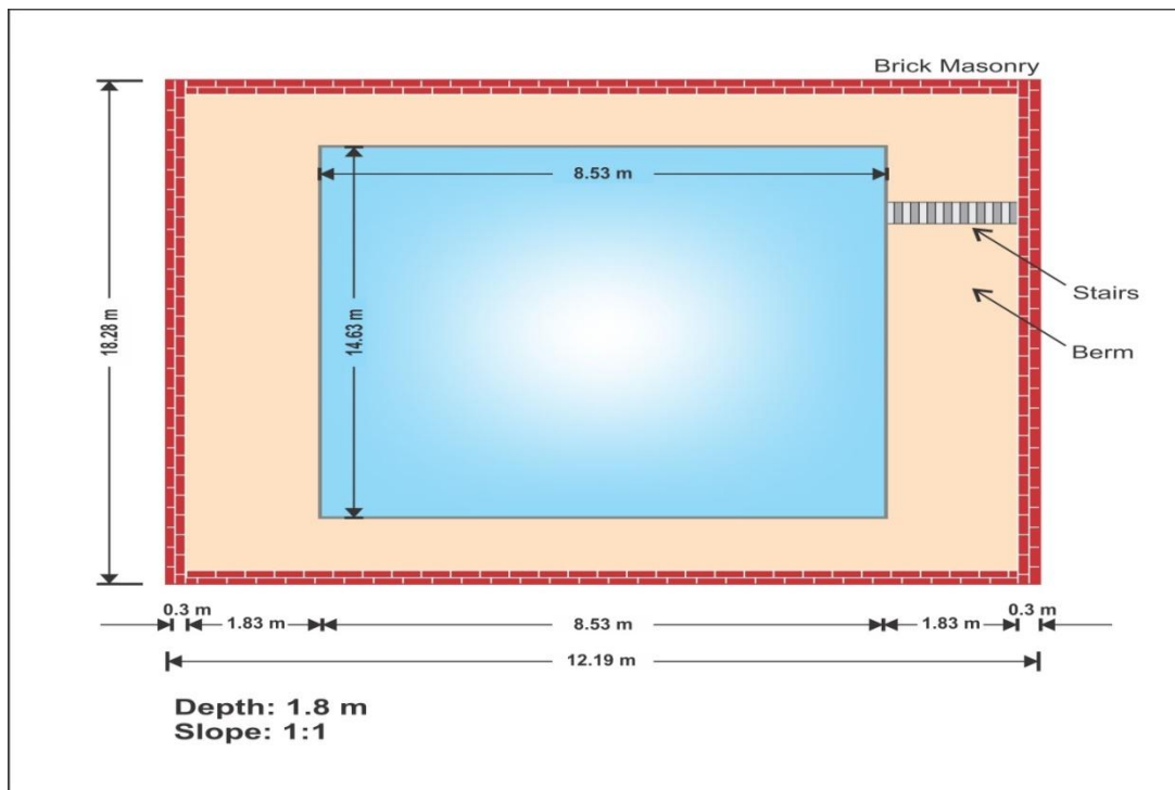
Figure 2: Schematic diagram of fish pond (Correct the dimensions; width (12.19m) is longer than width (18.28m) how?)
