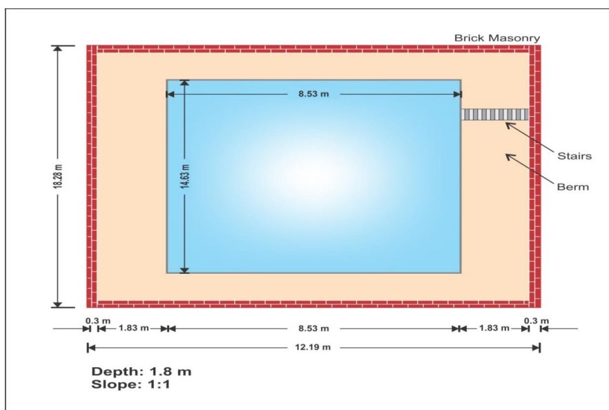
Figure 2: Schematic diagram of fish pond
