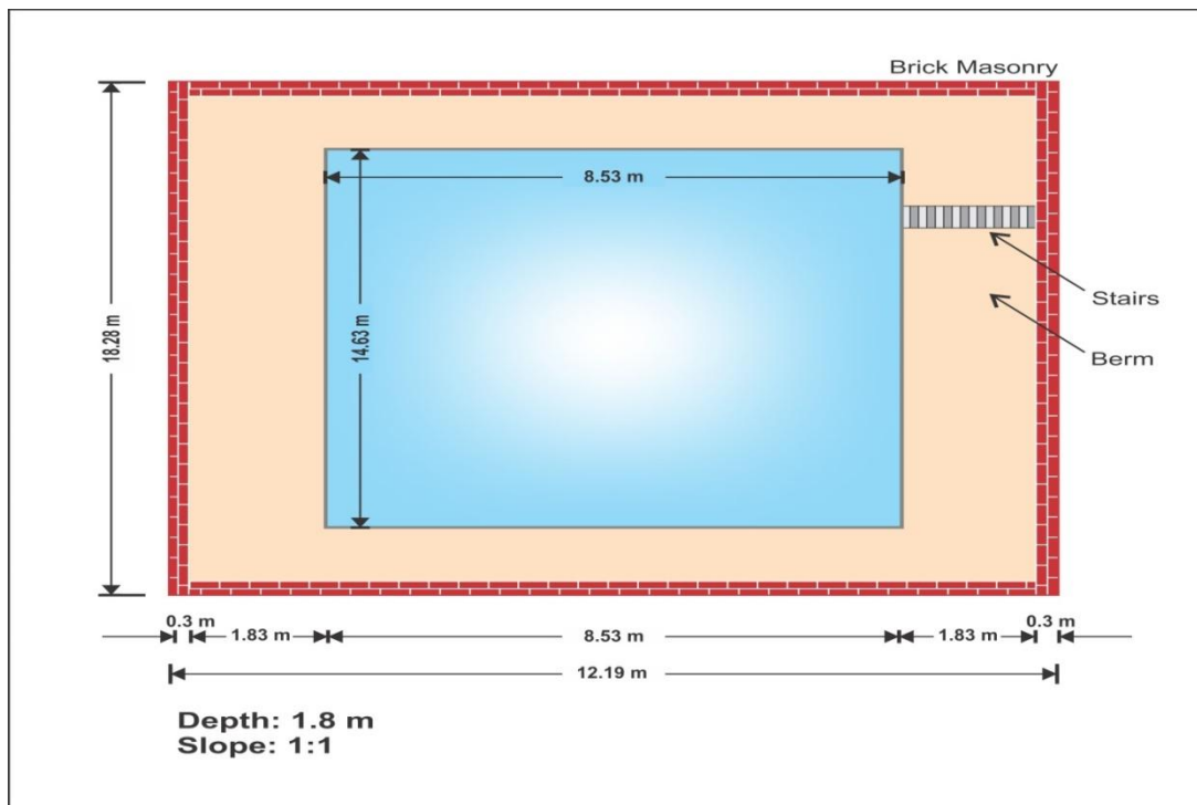
Figure 2: Schematic diagram of fish pond
