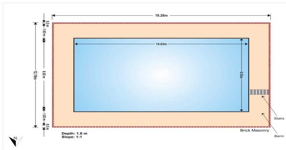
Figure 2: Schematic diagram of fish pond
