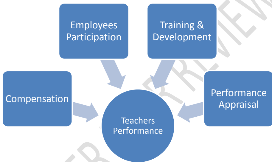
Fig 1. Research Framework
