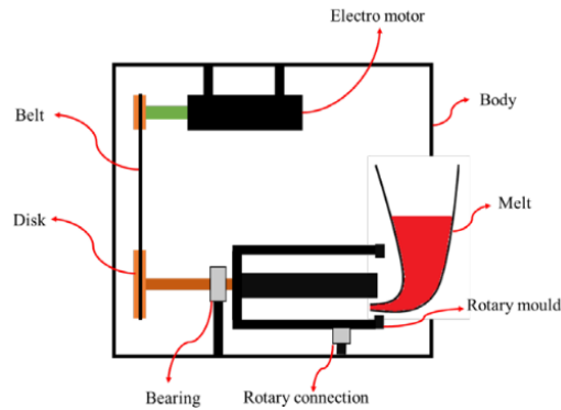
Figure. 1 Centrifugal Casting Process
