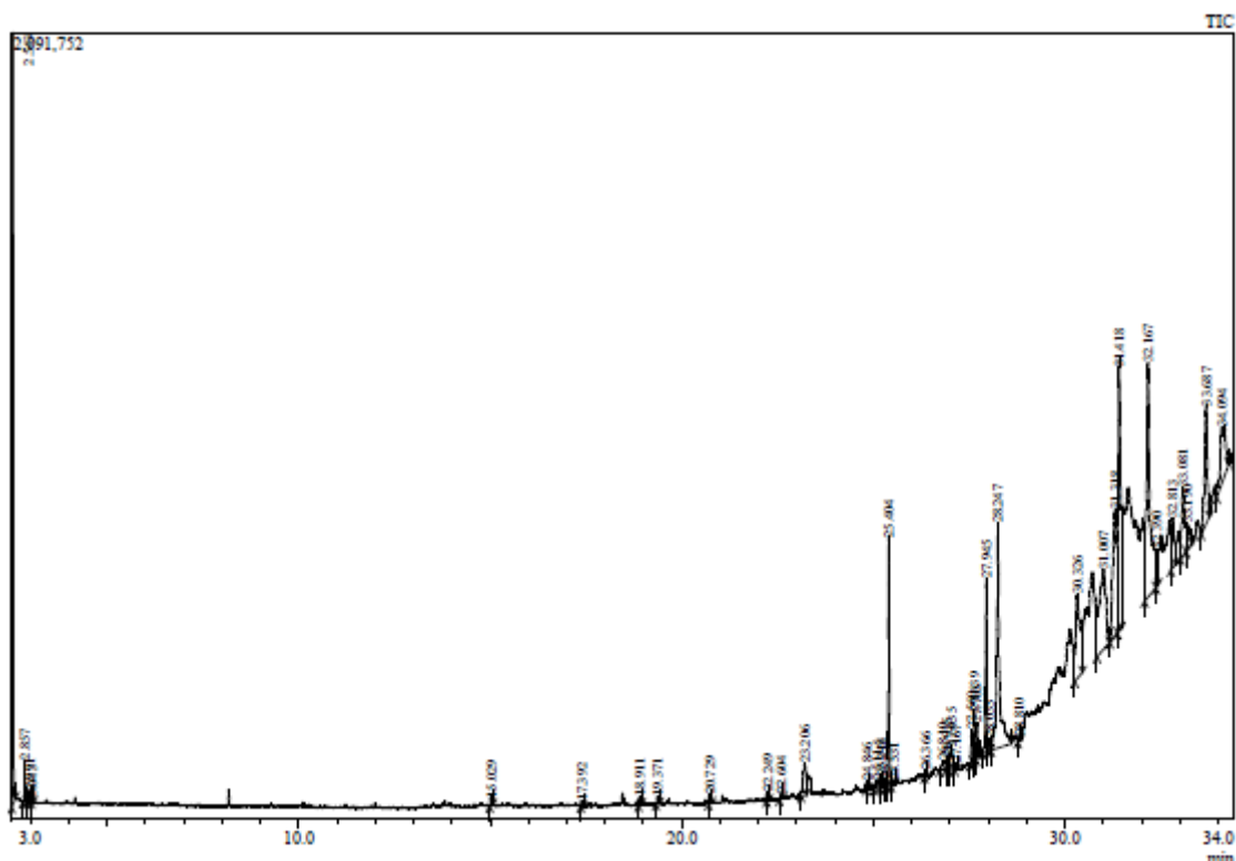
Figure 2: GC-MS Chromatogram of transesterified oil(FAME)
